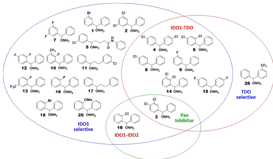
Figure 1. Venn diagram of selectivities seen with diaryl hydroxylamines in enzyme inhibition assay.
