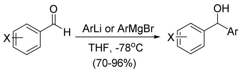
Scheme 1. Synthesis of Diaryl Alcohols with One Ring Substituted
