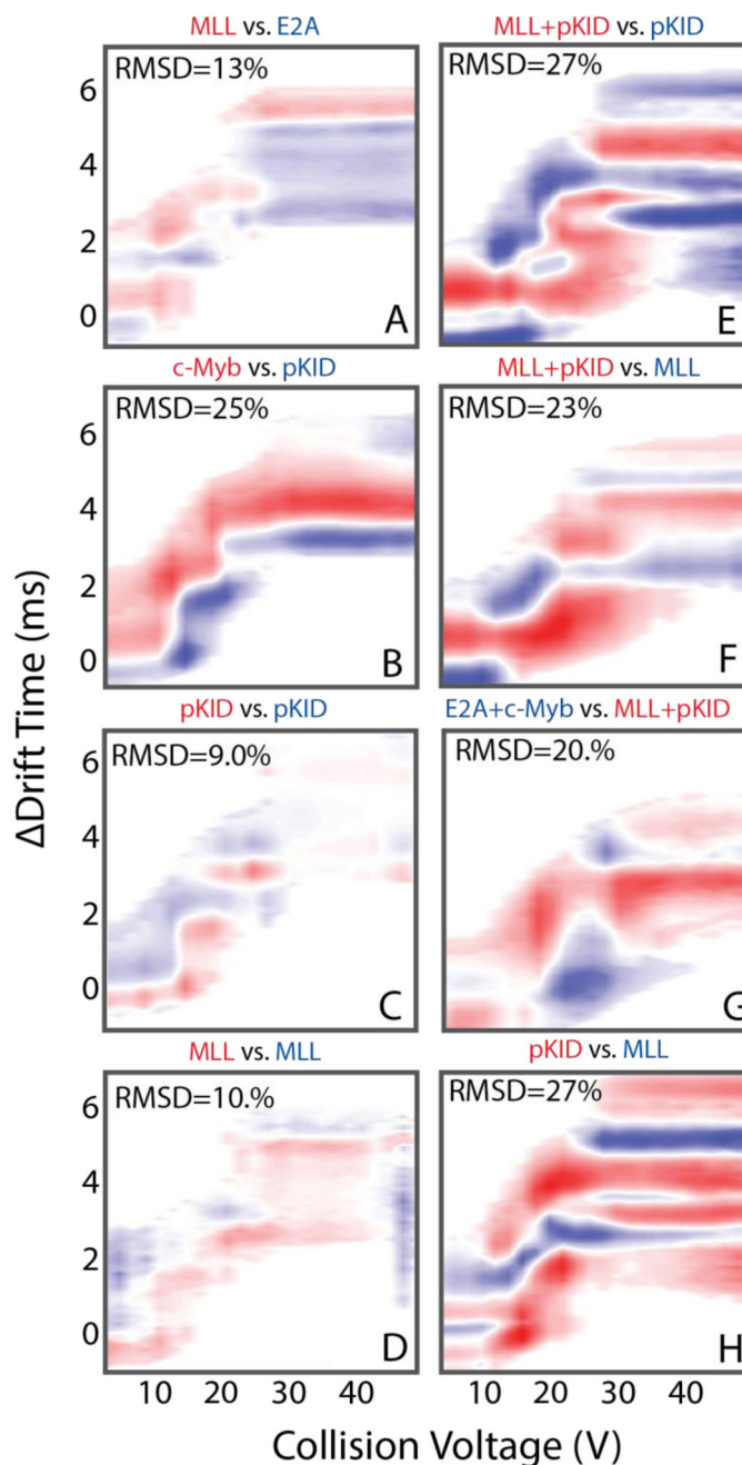
Figure 3. RMSD values and CIU difference plots, computed using CIUSuite, for binary comparison across the data shown in Figure 2. Each difference map indicates where the intensity values for the two subtracted CIU fingerprints are greatest with a blue/red color code, indicated above each panel. The comparisons made are between: (A) MLL and E2A KIX:peptide complexes, (B) pKID and c-Myb KIX:peptide complexes, (C) replicate KIX:pKID CIU fingerprints, (D) replicate KIX:MLL CIU fingerprints, (E) the ternary KIX:MLL:pKID complex and the KIX:pKID complex, (F) the ternary KIX:MLL:pKID complex and
