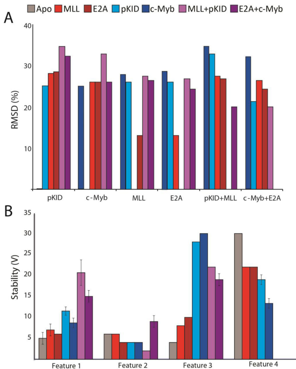
Figure 4. Histograms of the RMSD values and stabilities of the CIU features observed in Figure 2. (A) Histograms of the RMSD values from Figure 3 in histogram form. (B) A histogram of the CIU stability values recorded of each of the features observed in Figure 2.
