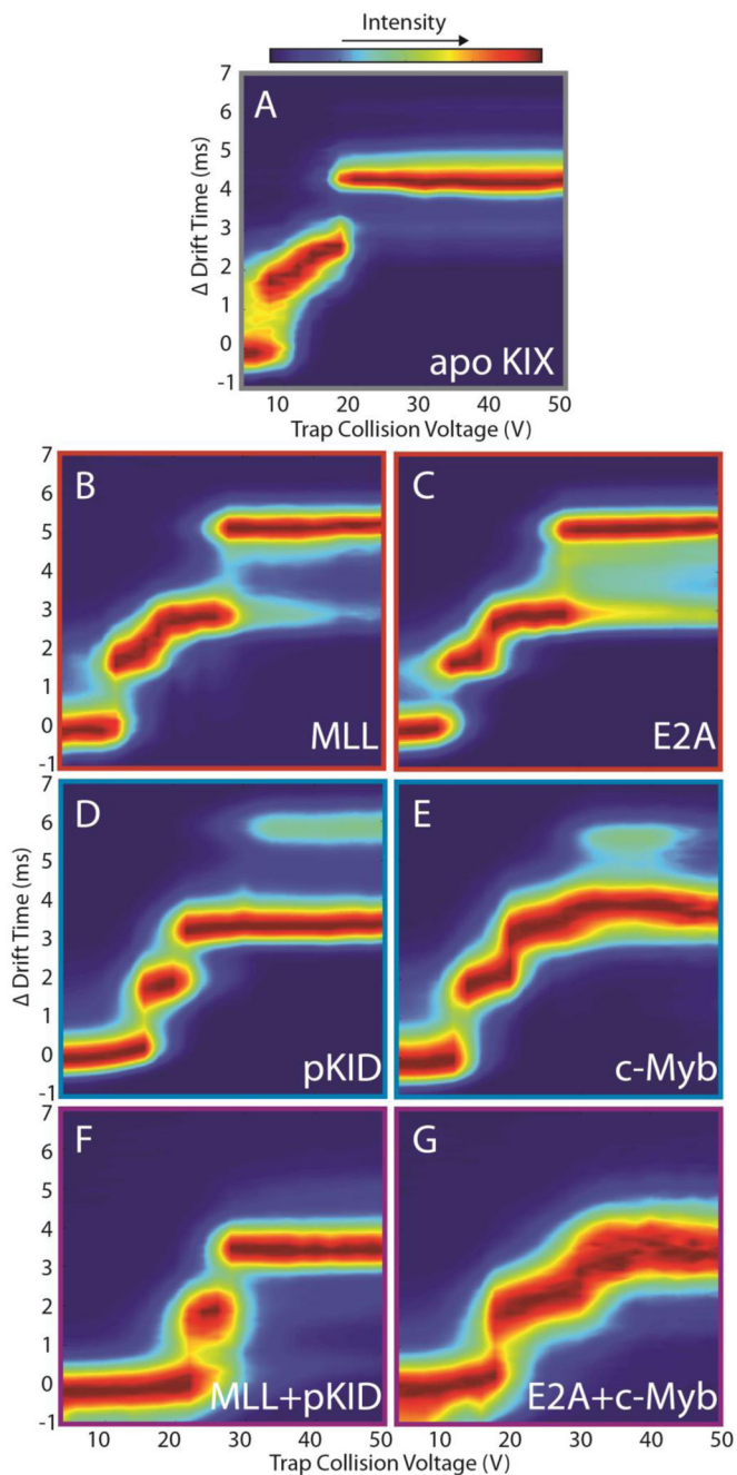
Figure 2. CIU fingerprints for the 8+ ions of the following KIX-associated proteins and complexes: (A) Apo KIX (B) KIX:MLL (C) KIX:E2A (D) KIX:pKID (E) KIX:c-Myb (F) KIX:MLL:pKID, and (G) KIX:E2A:c-Myb. Each of these CIU fingerprints is displayed on a drift time axis in order to facilitate comparisons across complexes having disparate starting sizes.
