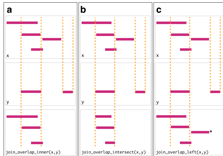
Fig. 2 Illustration of the three overlap join operators. Each join takes two GRanges objects, x and y as input. A “Hits” object for the join is computed which consists of two components. The first component contains the indices of the ranges in x that have been overlapped (the rectangles of x that cross the orange lines). The second component consists of the indices of the ranges in y that overlap the ranges in x . In this case a range in y overlaps the ranges in x three times, so the index is repeated three times. The resulting “Hits” object is used to modify x by where it was “hit” by y and merge all metadata columns from x and y based on the indices contained in the “Hits” object. This procedure is applied generally in the plyranges DSL for both overlap and nearest neighbor operations. The join semantics alter what is returned: a for an inner join the x ranges that are overlapped by y are returned. The returned ranges also include the metadata from the y range that overlapped the three x ranges. b An intersect join is identical to an inner join except that the intersection is taken between the overlapped x ranges and the y ranges. c For the left join all x ranges are returned regardless of whether they are overlapped by y . In this case, the third range (rectangle with the asterisk next to it) of the join would have missing values on metadata columns that came from y
