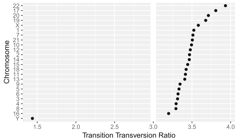
Fig. 5 The final result of computing quality control metrics over the SNP array data with plyranges , displayed as a dot plot. Chromosomes are ordered by their estimated transition-transversion ratio. A white reference line is drawn at the expected ratio for a human exome
