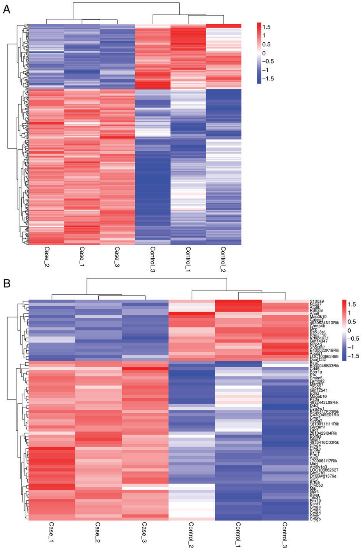
Figure 2. (A) Heat map of the differentially expressed lncRNAs for the DR group and control group. (B) Heat map of differentially expressed mRNAs for the DR group and control group. All the values were normalized to t values. In diabetic retina samples, 89 lncRNAs and 14 miRNAs were upregulated, whereas 214 lncRNAs and 3 miRNAs were downregulated. lncRNAs, long non-coding RNAs; DR, diabetic retinopathy; mRNAs, messenger RNAs; miRNAs, microRNAs.
