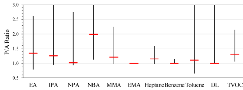
Figure 3. Personal/area (P/A) concentration ratios at 10th, 50th (red line) and 90th percentiles. (EA is ethyl acetate; IPA is isopropyl acetate; NPA is n-propyl acetate; NBA is n-butyl acetate; MMA is methyl methacrylate; EMA is ethyl methacrylate; DL is d-limonene.)
