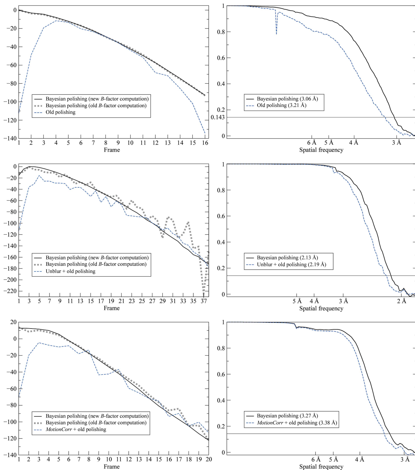
Figure 5 Comparison to previously published results for the ribosome (top), \beta -galactosidase (centre) and \gamma -secretase (bottom). Left: relative B factors. Unlike in Fig. 4, the vertical positions of these curves are arbitrary: only their shapes hold any meaning. The continuous black and dotted grey lines correspond to the same motion estimate, but they have been determined using the new and the old B -factor estimation techniques, respectively. Their similarity indicates that the new technique estimates the same B factors as the old technique, albeit in a more robust way. The dashed blue line corresponds to previously published B factors. Note the stark improvement at the beginning of the sequence. Right: FSC curves comparing the new results with the previously published results. Note that the old polishing approach estimated the motion as superimposed over that estimated by another, reference-free method, while Bayesian polishing always works on the raw unaligned micrographs and aims to model the entire motion by itself.
