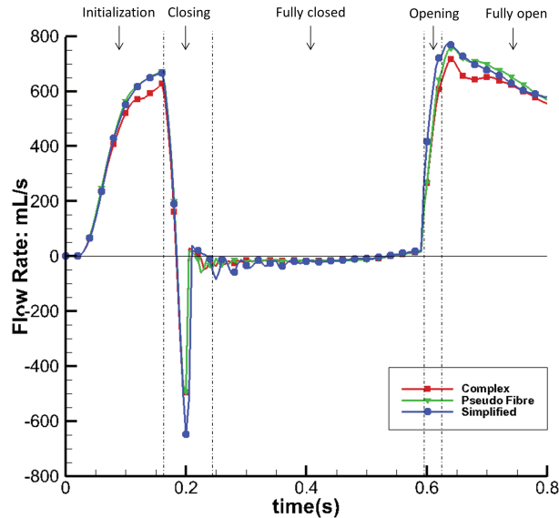
FIG. 11. Flow rate through the MV of the three different models.
