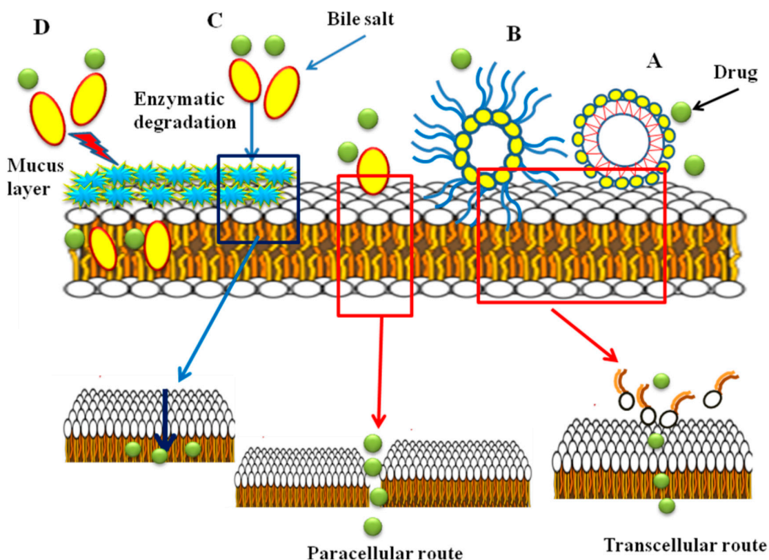
Figure 6. The most common transport mechanisms of bile salts; (A) micelle formation; (B) reverse micellization; (C) enzyme inhibition; (D) viscosity reduction of the mucus layer.
