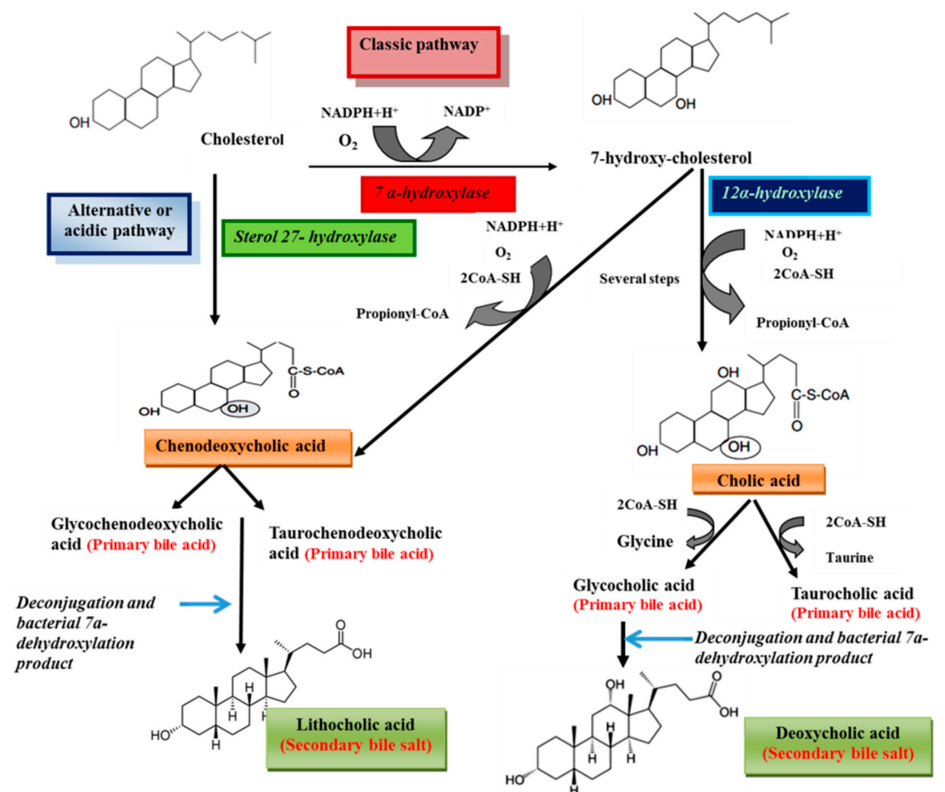
Scheme 1. Schematic representation of bile acids biosynthesis from cholesterol.
