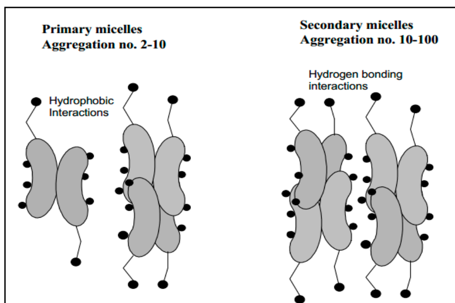
Figure 2. Primary and secondary aggregation model of bile salt micelles [18].
