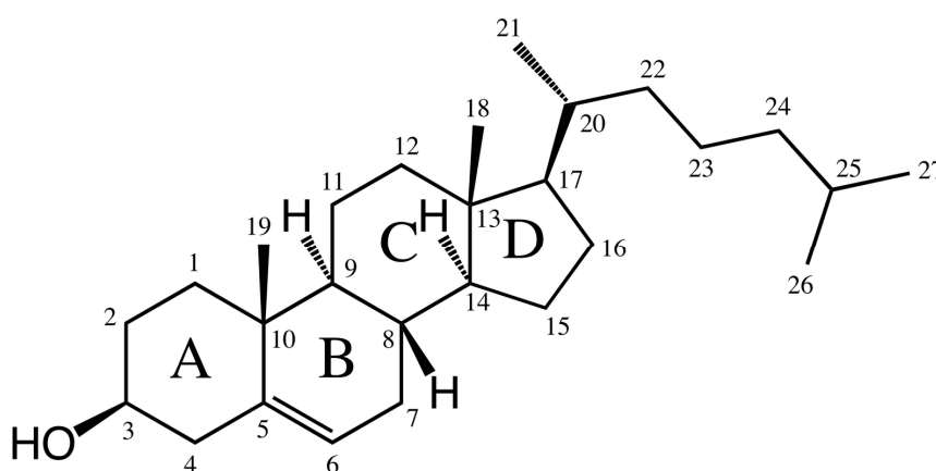
Figure 1. Common chemical structure of bile acids.
