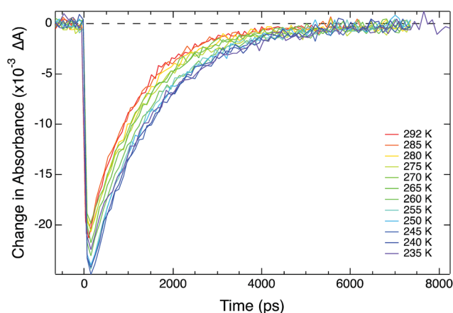
Fig. 3 Variable-temperature ground state recovery dynamics for [\text{Fe}(\text{bpy})_3]^{2+} in \text{CH}_3\text{CN} solution at 530 nm following ^1A_1 \rightarrow ^1MLCT excitation at 490 nm. The time constant increases from 1.05 \pm 0.02 ns at room temperature (red) to 1.52 \pm 0.03 ns 235 K (purple).
