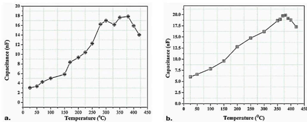
Figure 8. Capacitance-temperature ( C - T ) variations for the PZT/BiT films at 25–420 °C, (a) L 1 -A and (b) L 1 -B.
