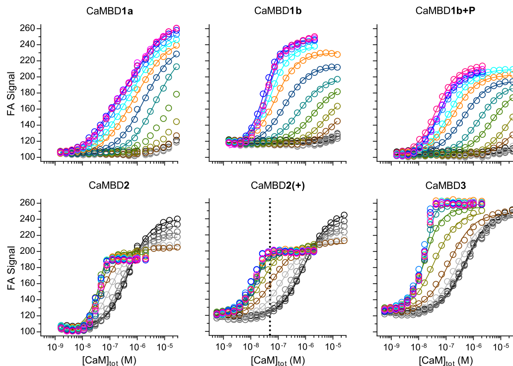
Figure 4. Example FA signal curves for the titration of RyR CaMBD peptides with CaM.
