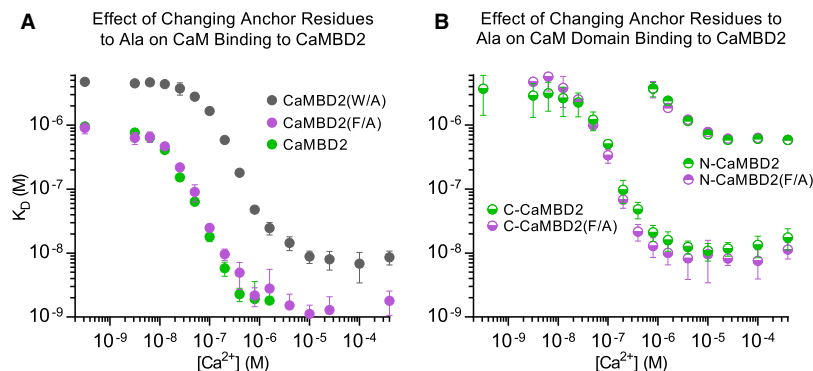
Figure 7. Effects of changing CaMBD2 Trp3587 and Phe3603 anchor residues to Ala on CaM binding. Effects of mutating RyR2 CaMBD2 anchor residues on the \text{Ca}^{2+} -dependent affinities of (A) full-length CaM and (B) N- and C-domains for binding to CaMBD2. The binding model-fitted affinities ( K_D ) are plotted as a function of [\text{Ca}^{2+}] . Note the double logarithmic axes. Error bars represent the 95% confidence intervals of two replicates.
