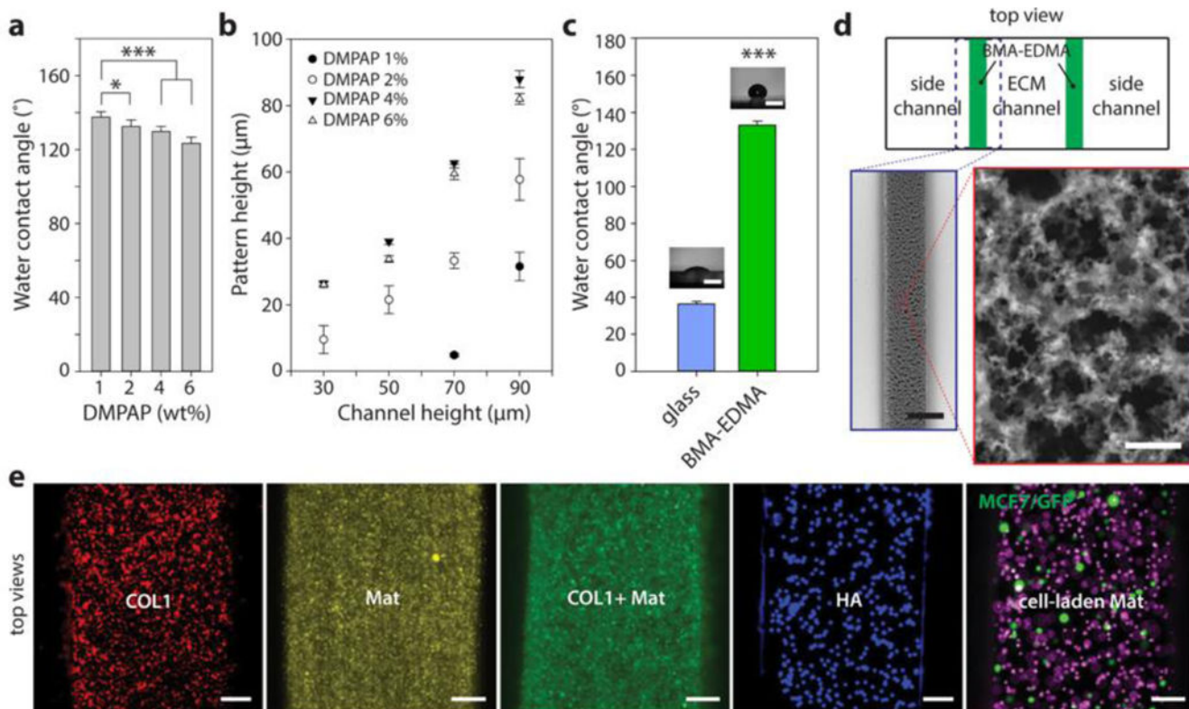
Figure 2. Characterization of BMA-EDMA and hydrogel patterning within the microfluidic device.
