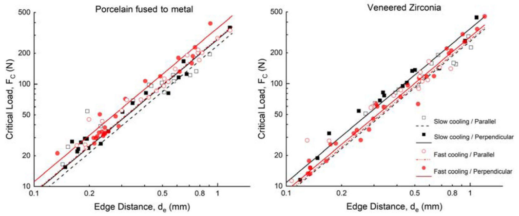
Figure 6. Plot of chipping load F_c versus indentation edge distance d . The lines represent the best fits of Eq. (2).
