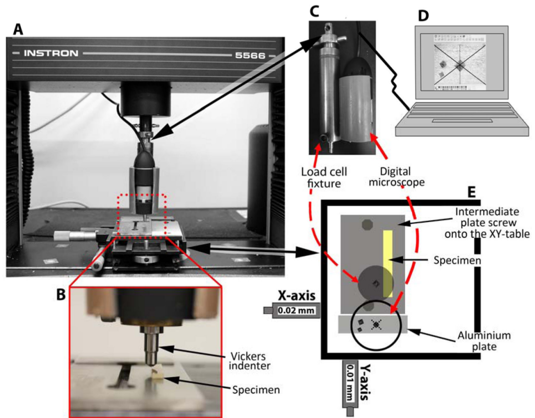
Figure 1. Edge chipping method. A: Universal testing machine setup. B: Enlarged specimen view. C: Side view of the load cell fixture coupled with the digital microscope. D: The digital microscope software view used to verify the indenter alignment setup. E: Top view of the XY-table coupled to the universal testing machine.
