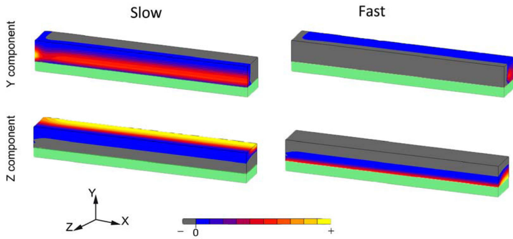
Figure 9. Thermal residual stress distribution, Y and Z components, in porcelain veneers cooled with the slow or fast protocol. Representation of \frac{1}{4} the specimen.
