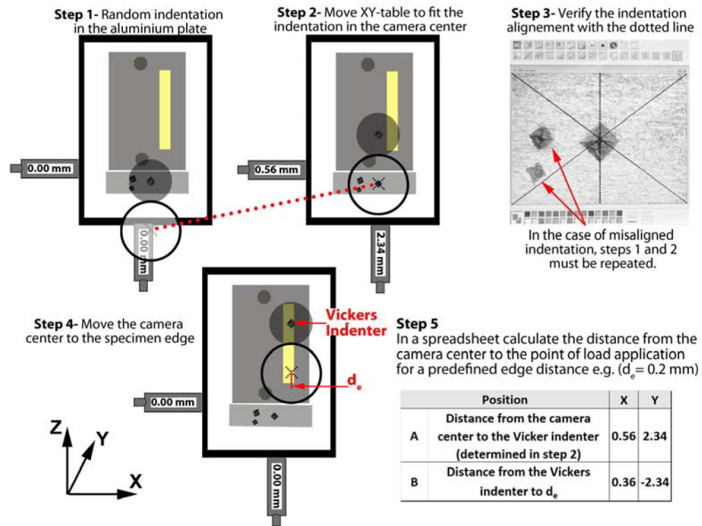
Figure 2. Steps to align the Vickers indenter with the specimen edge for the edge chipping procedure.
