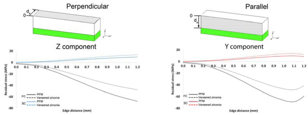
Figure 10. Y and Z components of the residual thermal stresses as a function of edge distance.
