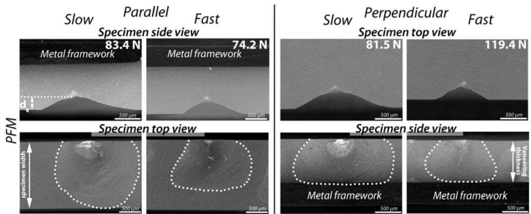
Figure 7. Chipping pattern for PFM specimens loaded with an edge distance of 0.5 mm. The dotted line delineates the chip outline in the top view for parallel loaded specimens and in the side view for perpendicularly loaded ones.
