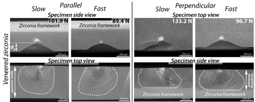
Figure 8. Chipping pattern for veneered zirconia specimens loaded with an edge distance of 0.5 mm. The dotted line delineates the chip outline in the top view for parallel loaded specimens and the side view for perpendicularly loaded ones.
