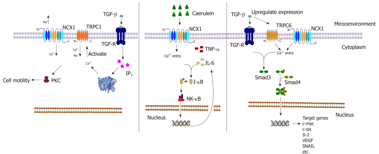
Figure 2 The regulated signal pathways and transcription factors of NCX1 in digestive diseases. Transforming growth factor- \beta (TGF- \beta ) stimulates the activation of PLC-IP 3 and Ca 2+ release from the endoplasmic reticulum, which activates TRPC1 and the reverse mode of NCX1 resulting in Ca 2+ influx, and the increase of Ca 2+ mediates cell motility directly or indirectly via activation of Ca 2+ -dependent PKC in pancreatic cancer. Cerulein activates NCX1 and induces activation of inflammatory factors TNF- \alpha and IL-6 and the downstream NK- \kappa B pathway in pancreatic cells. TGF- \beta can upregulate the expression of NCX1 and TRPC6 and activate the downstream SMAD pathway to regulate the migration and invasion of hepatocellular carcinoma cells.
