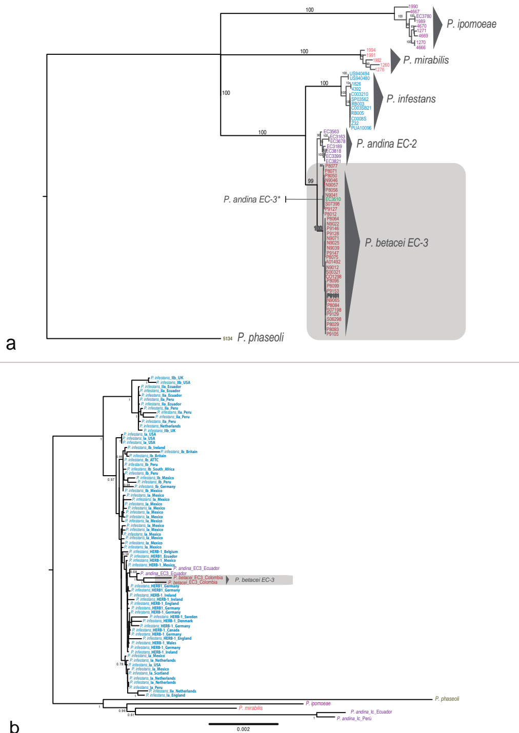
Fig. 1 Phylogenetic relationships of the Phytophthora betacei isolates and the closely related species, based on genotyping by sequencing (GBS) data and phylogeny of complete mitochondrial genomes. a. The tree was inferred using maximum likelihood (ML) with P. phaseoli as an outgroup. Support values associated with branches correspond to ML bootstrap support values (BS); b. ML phylogeny of complete mitochondrial genomes showing the phylogenetic position of P. betacei sp. nov. Only bootstrap support values above 50 % are shown.
