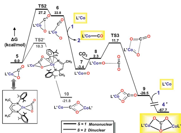
Fig. 6 M06L/def2-TZVPP Gibbs free energy ( \Delta G ) profile for the mononuclear dissociative pathway. Isolated species are shown in yellow boxes, with L' depicted instead of L'^{\text{tBu}} . *Marked species has lower relative free energy on the S = 3 surface which has been taken to complete the profile.
