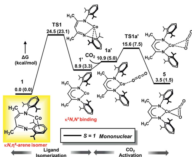
Fig. 4 Computed DLPNO-CCSD(T)/def2-TZVPP Gibbs free energy ( \Delta G ) profile for isomerization of 1 ( L'Co ) to 1' followed by CO 2 activation. Relative free energy values (in kcal mol -1 ) computed with M06L/def2-TZVPP are given in parentheses. The isolated species is shown in the yellow box, with L' depicted instead of L^{tBu} .
