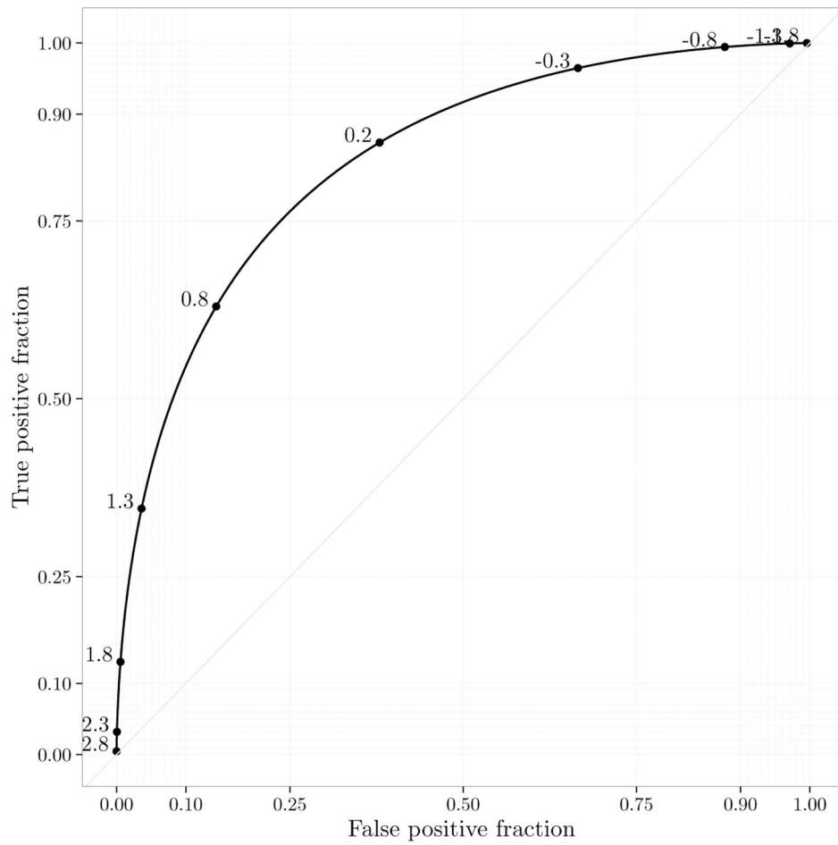
Figure 7: Illustration of smooth binormal ROC curve.
