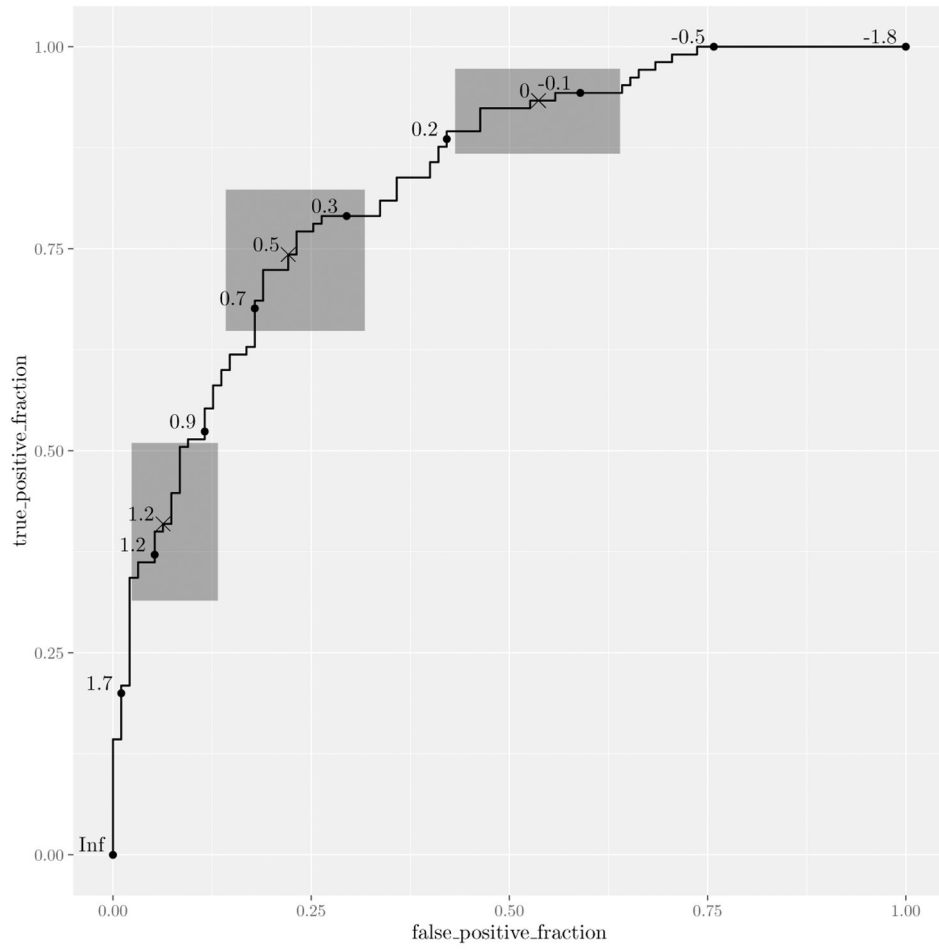
Figure 2: Illustration of plotROC with exact confidence regions.
