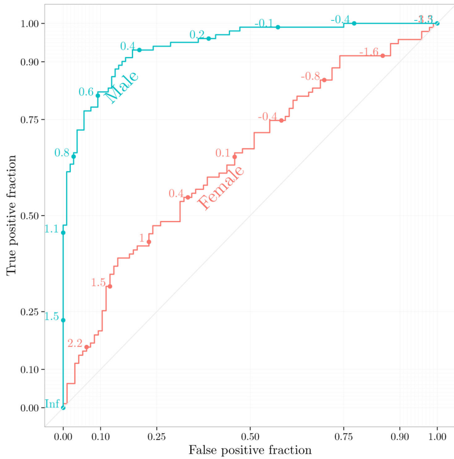
Figure 5: Illustration of plotROC with multiple curves.
