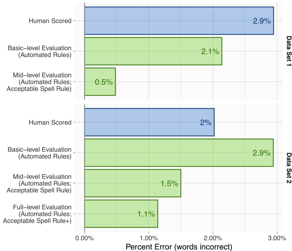
FIG. 2. (Color online) The error rates of scoring orthographic listener transcripts for a measure of words correct for Autoscore and human scorers for both in-house data sets.
