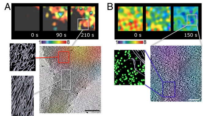
Fig. 3. Time evolution of Rac1 activity defined at the nanoscale. (A) Molecular organization of cytoskeleton assemblies at actively protruding filopodium. (Upper) Successive images of Rac1 activity near the base of an actively extending filopodium, taken from live-cell ratio imaging of an MEF cell. (The width of each box is 3 \mu\text{m} .) The pseudocolor scale shows the increase in ratio relative to the lowest 5% of ratio values in the cell. (Lower) The last time frame captured by cryo-ET. Regions with high Rac1 activity (Upper, dark-gray box) show the characteristic short actin filament morphology with little directional alignment. Note the appearance of the characteristic morphology of filopodial bundle (Lower, light gray box) at close spatial proximity. (Scale bar, 300 nm.) (B) Molecular organization of cytoskeleton assemblies at site of lowering Rac1 activity. (Upper) Successive images of a region taken from live-cell ratio imaging of an MEF cell. (The width of each box is 3 \mu\text{m} .) The pseudocolor scale shows the increase in ratio relative to the lowest 5% of ratio values in the cell. The region turned from primarily high Rac1 activity (red) to low Rac1 activity (purple/blue) within 150 s. (Lower) The last time frame captured by cryo-ET. The region is dominated by ribosomes interspersed with long, aligned actin filament and vesicular assemblies. Short actin filaments, characteristic of regions with high Rac1 activity, are no longer present, suggesting that, in less than 150 s this morphology is replaced. (Scale bar, 150 nm.)
