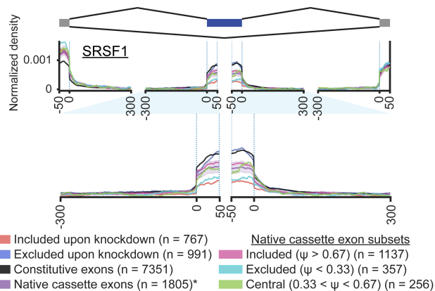
FIGURE 5. Choice of background affects interpretation of splicing maps. Lines indicate average normalized eCLIP signal at SRSF1 (red) knockdown-included and (blue) knockdown-excluded cassette exon events against four controls: constitutive exons (with no exclusion reads across multiple control RNA-seq data sets), native cassette exons with 0.05 < \text{percent spliced in } (\Psi) < 0.95 in at least half of ENCODE control RNA-seq data sets, and subsets of native cassette exons with average \Psi < 0.33 (excluded), 0.33 < \Psi < 0.67 (central), and \Psi > 0.67 (included) in ENCODE control RNA-seq data sets.
