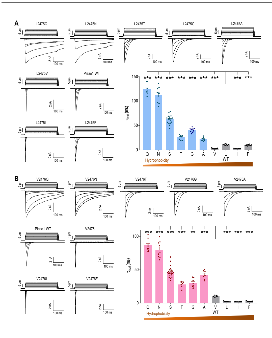
Figure 3. The hydrophobicity of L2475 and V2476 determines the rate of Piezo1 inactivation. ( A and B ) Representative whole-cell MA current traces and quantification of MA current inactivation rate ( \tau_{inact} ) in HEK293T AP1 cells expressing Piezo1 with indicated mutations of variable hydrophobicity at L2475 ( A , n = 7-18 cells) and V2476 ( B , n = 6-22 cells). E_{hold} = -80 mV. ** p < 0.01 , *** p < 0.001 , one-way ANOVA with Holm-Sidak's correction. Data are mean \pm SEM.
