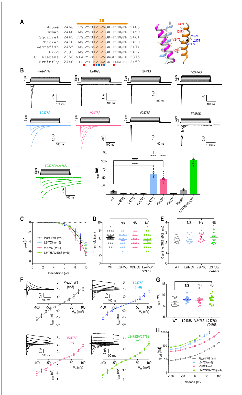
Figure 2. The pore-lining inner helix plays a major role in Piezo1 inactivation. (A) Left panel, amino acid sequence alignment of the Piezo1 inner helix (IH) from different species. A cluster of five conserved hydrophobic residues in the middle are highlighted. Red and blue dots indicate hydrophobic residues facing and pointing away from the pore, respectively. Right panel, cryo-EM structure of the Piezo1 inner helix (PDB: 6BPZ) showing the hydrophobic residues in the left panel. (B) Representative whole-cell MA current traces and quantification of MA current inactivation rate ( \tau_{inact} ) in Figure 2 continued on next page
