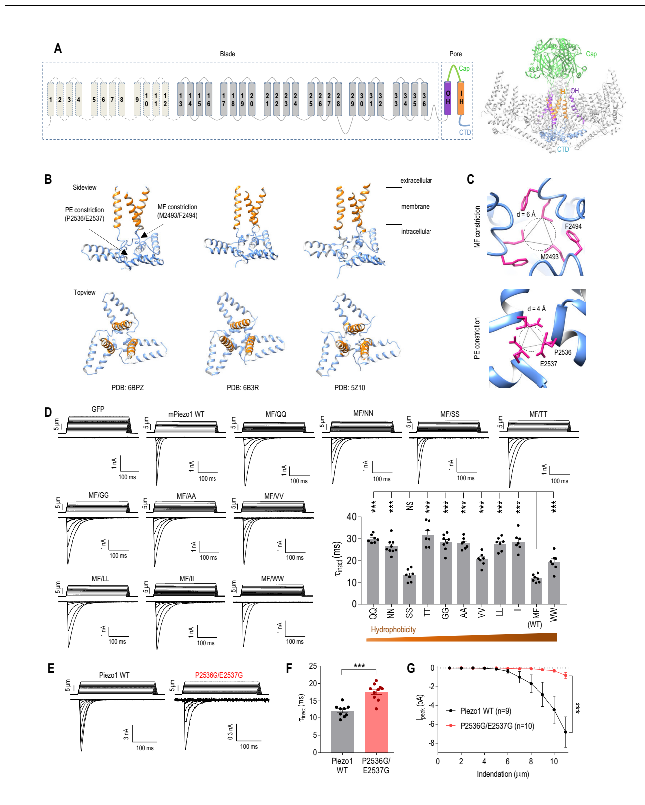
Figure 1. Physical constrictions in the CTD play only moderate roles in Piezo1 inactivation. (A) Topology diagram and cryo-EM structure of Piezo1 (PDB: 6BPZ). IH, inner pore helix; OH, outer pore helix. (B) Side view and top view of the Piezo1 pore region from three cryo-EM structures showing the location of the MF and PE constrictions. (C) Top view close-up of the MF and PE constrictions in Piezo1 (PDB: 6BPZ). (D) Representative whole-cell MA current traces and quantification of MA current inactivation rate ( \tau_{inact} ) in HEK293T AP1 cells expressing Piezo1 with mutations at the M2493 F2494 (MF) Figure 1 continued on next page
