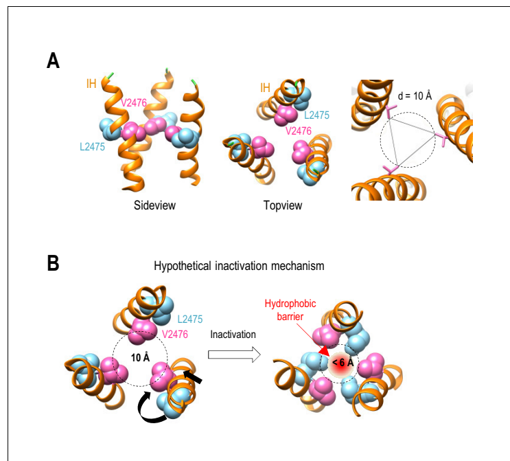
Figure 6. Hypothetical inactivation mechanism of Piezo1. (A) Left and middle panels, the side view and top view of a portion of Piezo1 inner helix (PDB: 6BPZ) showing the orientations of L2475 and V2476 residues with respect to the ion permeation pore. Right panel, pore diameter at V2476. (B) A hypothetical mechanistic model for Piezo1 inactivation at the hydrophobic gate in the inner helix. Inactivation is proposed to involve a combined twisting and constricting motion of the inner helix (black arrows), allowing both V2476 and L2475 residues to face the pore to form a hydrophobic barrier.
