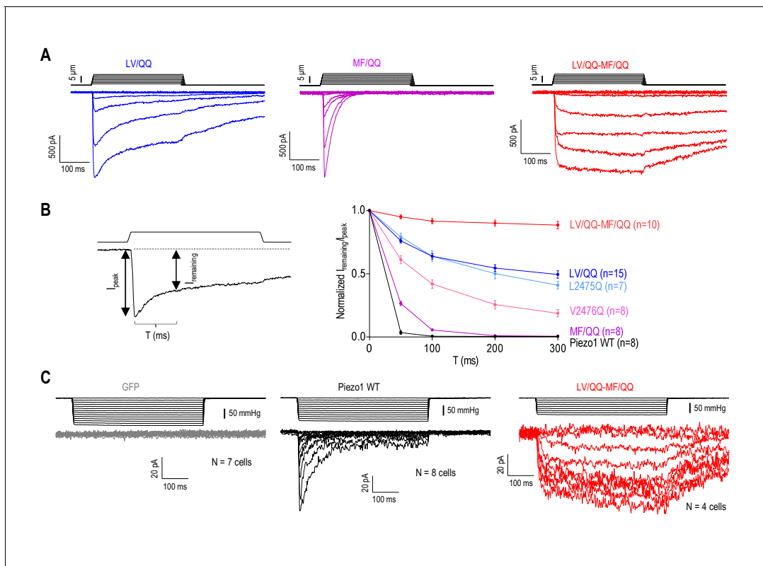
Figure 4. Mutation of the inner helix and MF constriction eliminates Piezo1 inactivation. (A) Representative whole-cell MA current traces from HEK293T \Delta P1 cells expressing Piezo1 with glutamine mutations in the putative hydrophobic gate (L2475/V2476, LV), or the MF constriction (M2493/F2494, MF). E_{\text{hold}} = -80 mV. (B) Left panel, an example trace of Piezo1 MA current illustrating the measurement of the ratio of remaining MA current amplitude ( I_{\text{remaining}} ) to peak ( I_{\text{peak}} ) at different time points during current decay. Right panel, quantification of I_{\text{remaining}}/I_{\text{peak}} for WT or mutant Piezo1. Data are mean \pm SEM. (C) Representative cell-attached MA current traces induced by high-speed pressure clamp via application of a negative pipette pressure in HEK293T \Delta P1 cells expressing GFP (negative control), WT or mutant Piezo1. E_{\text{hold}} = -80 mV.
