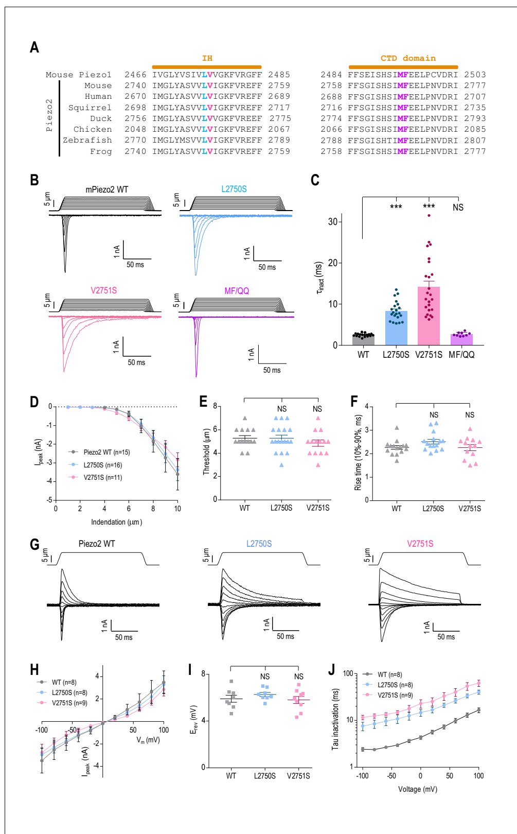
Figure 5. The putative inner helix inactivation gate is functionally conserved in Piezo2. (A) Amino acid sequence alignments of the IH and part of CTD between mouse Piezo1 and Piezo2 orthologues from indicated species. The conserved L2475 and V2476 residues in the IH are highlighted in blue and red; M2493 and F2494 in the CTD are highlighted purple. (B and C) Representative whole-cell MA current traces of WT and mutant Piezo2 (B), and Figure 5 continued on next page
