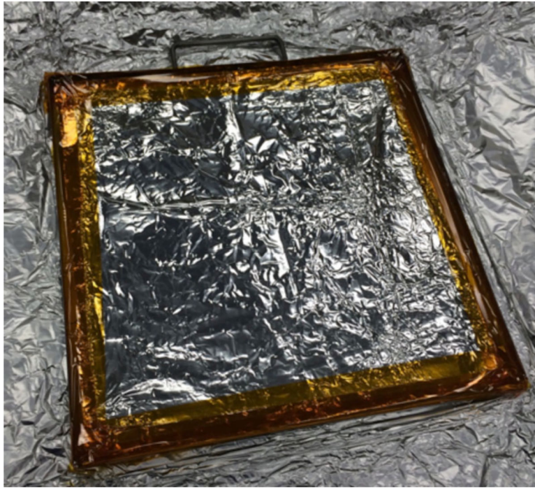
Fig. 5. Amino acid contamination monitoring plate adapted from a standard 1 \times 1 ft. ASTM E1235–12 NVR plate for the 4-m Atlas V fairing
