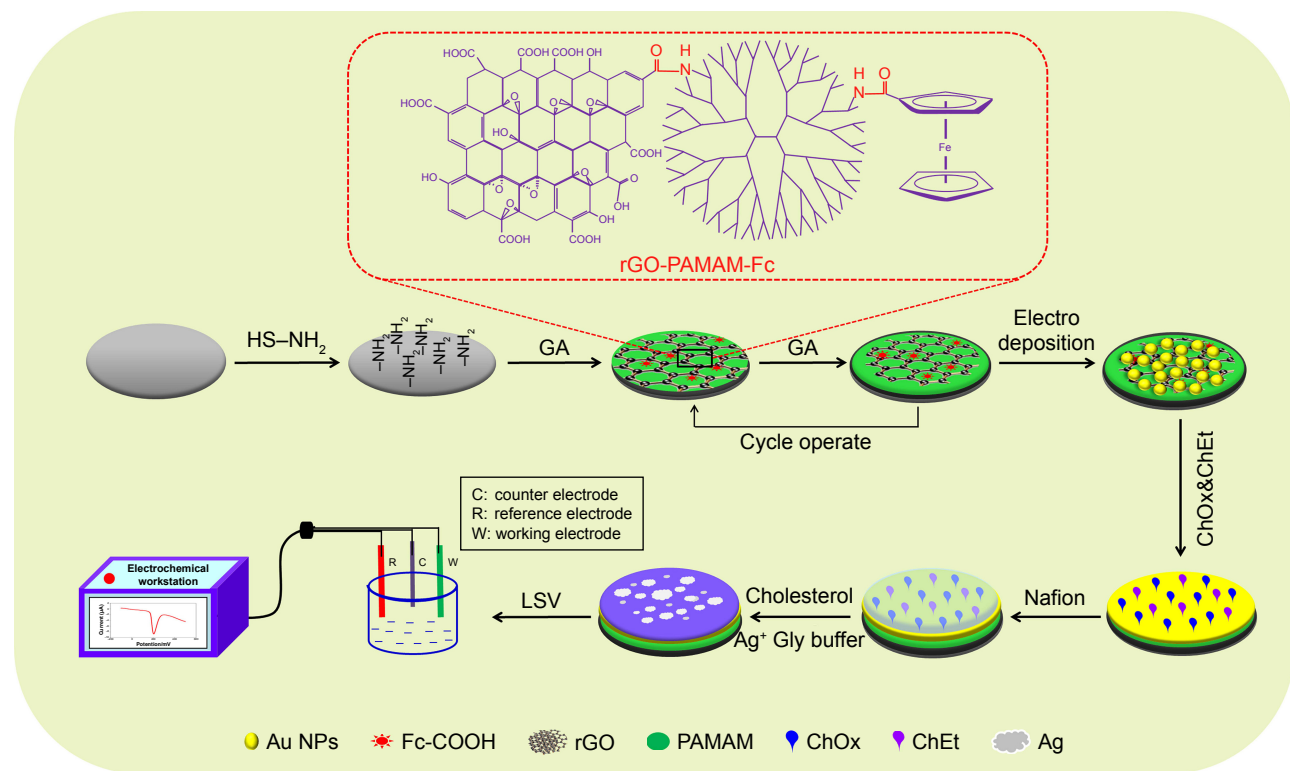
Scheme 1 Principle of ChOx&ChEt/Au NPs/rGO-PAMAM-Fc biosensor detecting cholesterol.
