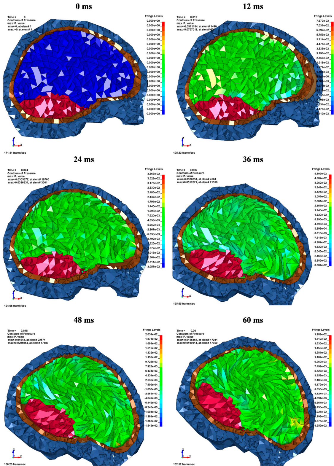
Figure 7. Head kinematics during the C755-T2 numerical test, with the cross-section in the median plane and showing the hydrostatic pressure (MPa) in the cerebrum.
