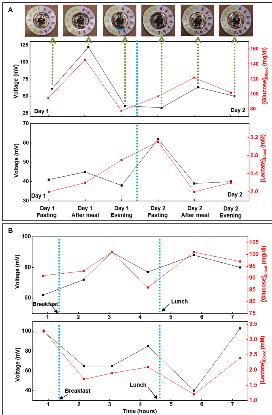
Fig. 7. Human trails. Correlation of data acquired from biofuel cell-based glucose and lactate sweat sensors with that acquired from blood glucose and lactate meters, respectively, over a period of (A) 2 days and (B) 1 day for subject #1 (with time lag compensation). Photo credit: Philipp Gutruf, Northwestern University.
