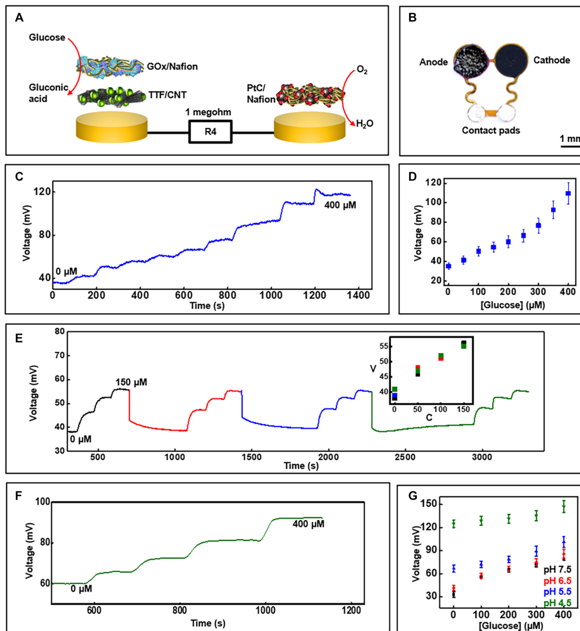
Fig. 4. Glucose sensor characterization. (A) Exploded-view schematic illustration of the layer makeup of the biofuel cell–based glucose sensor. GOx, glucose oxidase; PtC, platinumized carbon. (B) Image of the glucose sensor. (C) Real-time sensor response to increasing glucose concentration in phosphate buffer (pH 7.0) at 25°C and (D) the corresponding calibration ( n = 3 ). (E) Plot illustrating the reversible response of the glucose sensor for four consecutive cycles of varying glucose concentration. V, voltage in millivolts; C, concentration in micromolar. Inset shows calibration plot comparing the sensor signal plotted in (E) for the four cycles. (F) Real-time data acquired with increasing glucose concentration in artificial sweat under common physiological sweat conditions [temperature, \sim 30^\circ\text{C} (pH 5.5)]. (G) Calibration plot obtained from glucose sensors at \sim 30^\circ\text{C} in artificial sweat with different pH ( n = 3 ). Photo credit: Philipp Gutruf, Northwestern University.
