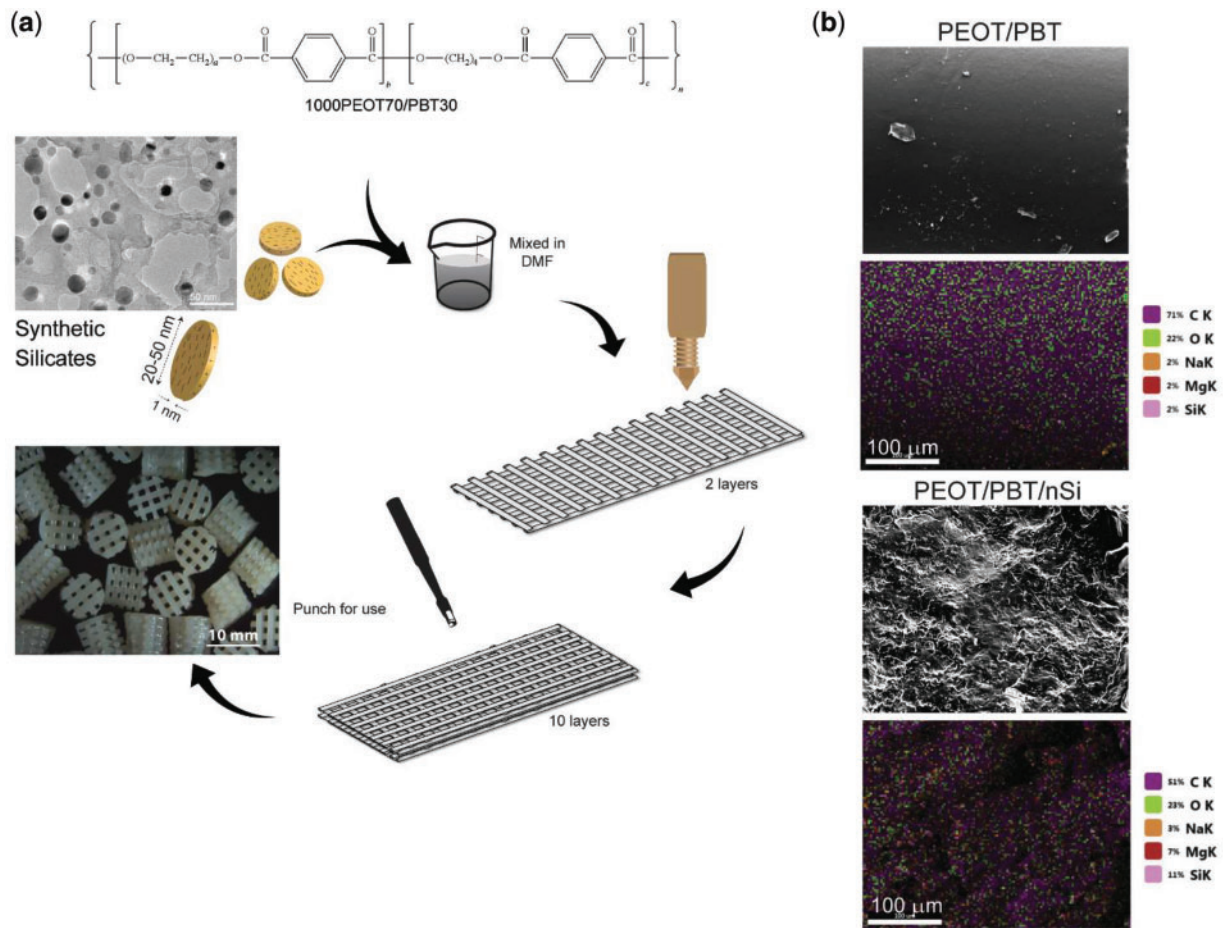
Figure 1. Fabrication of 3D nanocomposite scaffolds. (a) The addition of PEOT/PBT and nanosilicates in DMF resulted in a homogeneous solution for extrusion; (b) EDS analysis indicated an increase of mineral-specific elements following introduction of nanosilicates throughout the 3D structure
