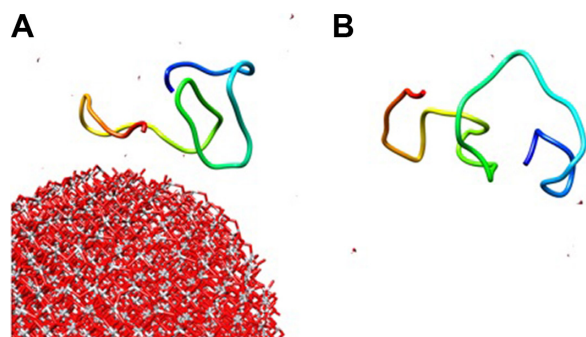
Figure 12 The molecular dynamic study of 2MZ7 segment in the presence (A) and absence (B) of \text{TiO}_2 cluster after 300 ps evolution.
