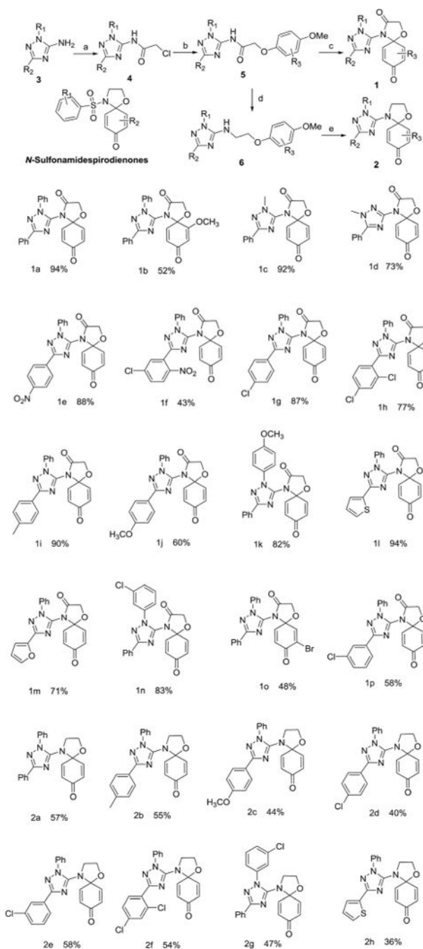
Fig. 1. N -Sulfonamide spirodienones and synthetic scheme of designed novel triazole-spirodienone conjugates (1 and 2). Reagents and conditions: (a) chloroacetyl chloride, (Et) 3 N, CH 2 Cl 2 ; (b) R 3 -PhONa, DMF; (c) [Cu(CH 3 CN) 4 ]ClO 4 , PhI(CF 3 CO 2 ) 2 , CH 2 Cl 2 , rt; (d) LiAlH 4 , AlCl 3 ; (e) Cu(CF 3 SO 2 ) 2 , PhI(CF 3 CO 2 ) 2 , CH 2 Cl 2 , rt.
