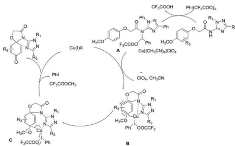
Scheme 2. Proposed mechanism for oxidative amination.
