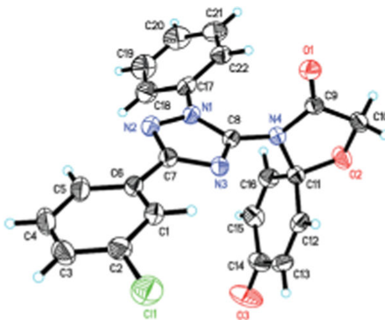
Fig. 2. ORTEP plot of molecular structure of 1p .
