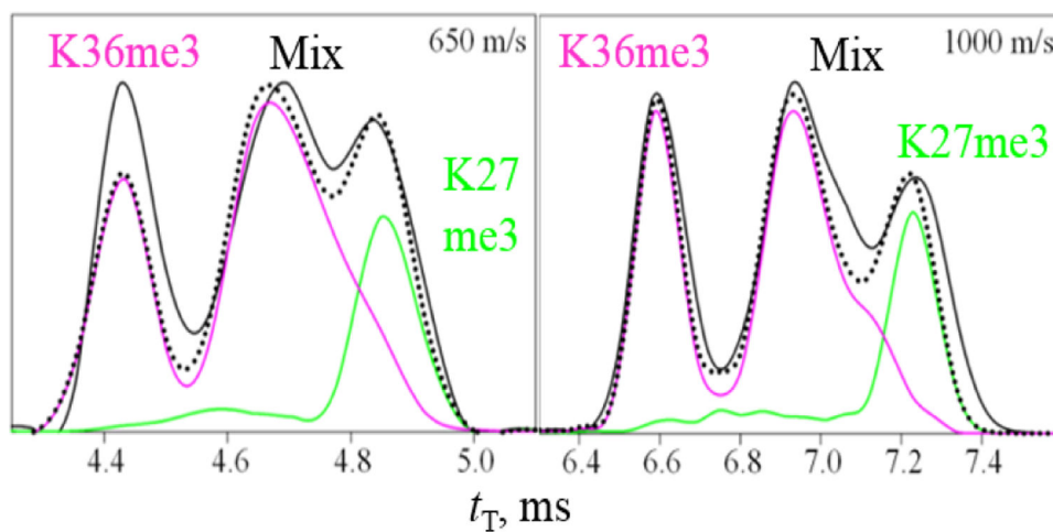
Figure 3. TWIMS spectra for K27me3/K36me3 mix ( z = 9 ) measured with solvent (i) depending on the waveform speed (solid black lines), with fits by scaled individual traces (colored lines) and their computed sum (dotted lines). Data for other speeds and mixtures are in Figure S3.
