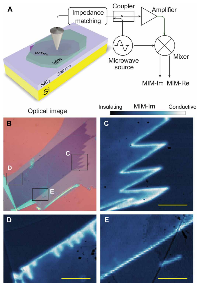
Fig. 1. Imaging edge conductivity in monolayer WTe 2 . (A) Schematics of the technique and device structure. (B) Optical image of a WTe 2 monolayer exfoliated onto SiO 2 and covered with a 10-nm-thick hBN. (C to E) MIM-Im images of the regions marked in (B), measured at T = 8 K and B = 0 . Scale bars, 5 \mu\text{m} .
