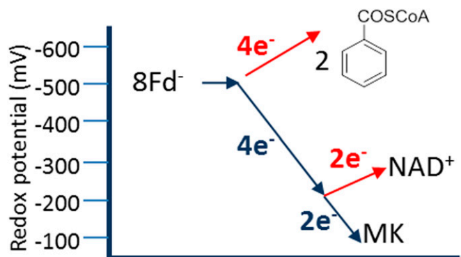
Fig. 5. Schematic scenario for double FBEB processes driving benzoyl-CoA reduction by class II BCRs. Red and dark blue arrows indicate endergonic and exergonic electron transfer reactions, respectively.
