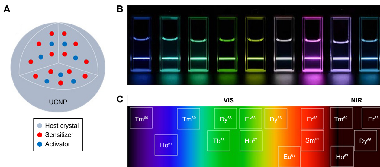
Figure 2 UCNP characteristics.
