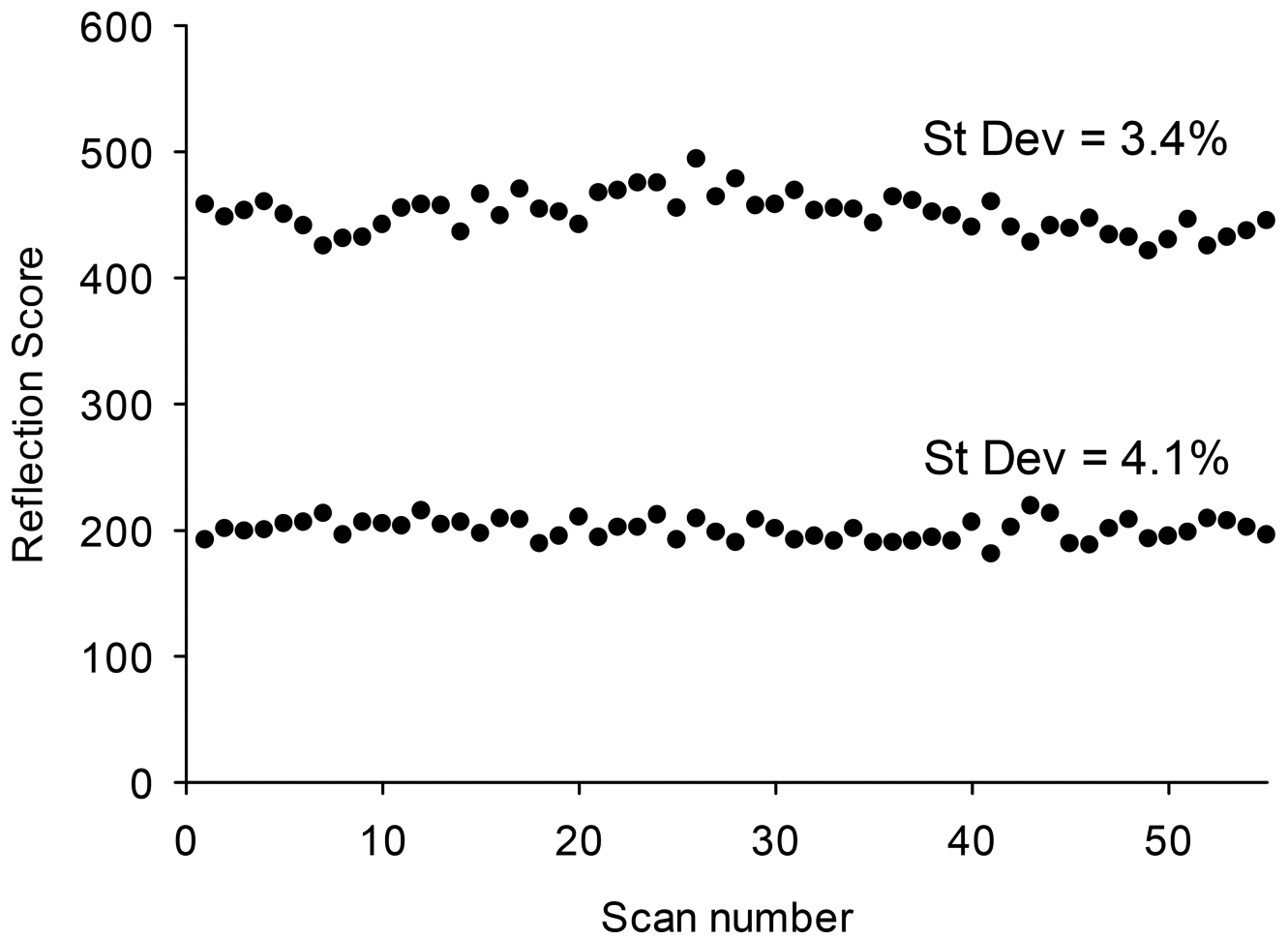
Fig. 5. Repeatability of RS skin carotenoid scores, comparing two subjects with relatively high score (a) and low score (b). Average scores were 460 and 200, respectively, with corresponding standard deviations of 3.4 and 4.1%. The standard deviation increases with lower score, consistent with the reduced signal to noise level.
