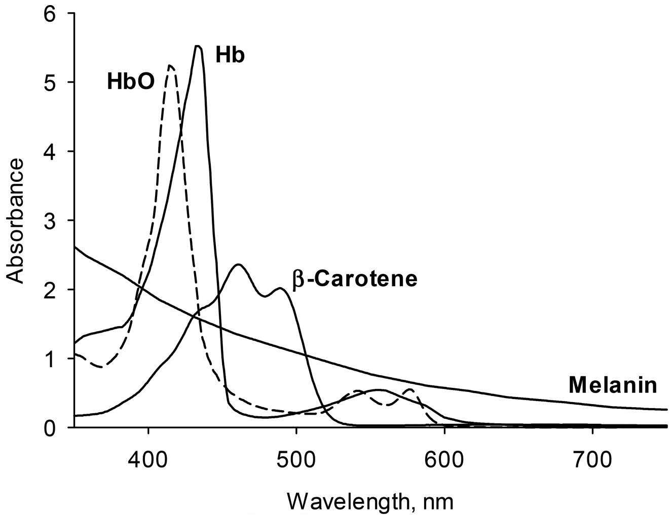
Fig. 1. Schematic absorption spectra of chromophores in human skin, including transitions from oxy- hemoglobin, HbO, de-oxyhemoglobin, Hb, \beta -carotene, and melanin. A spectral window for the detection of carotenoids with relatively weak absorptions from Hb/HbO exists in the 460–520 nm wavelength range.
