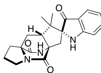
(+)-Brevianamide B (9)
