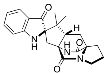
(+)-Brevianamide A (8)
