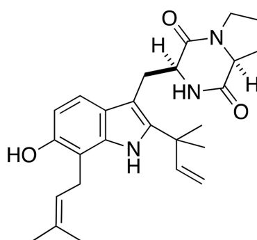
Notoamide S (13)
