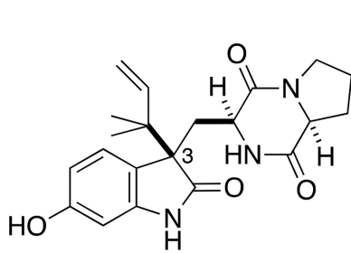
Notoamide J (10)
