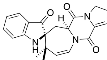
Austamide (14)
