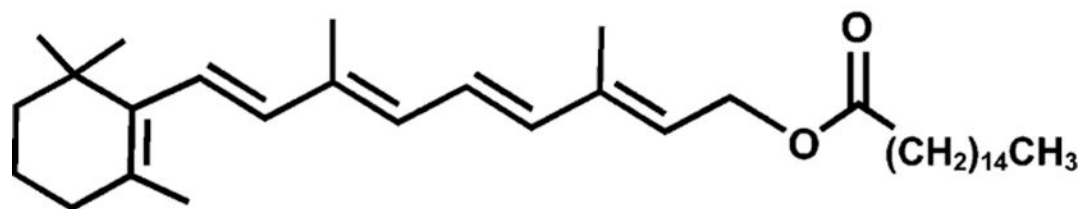
Retinyl Palmitate (RP)
