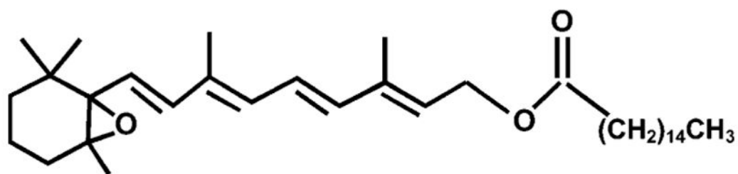
5,6-Epoxyretinyl Palmitate (5,6-Epoxy-RP)
