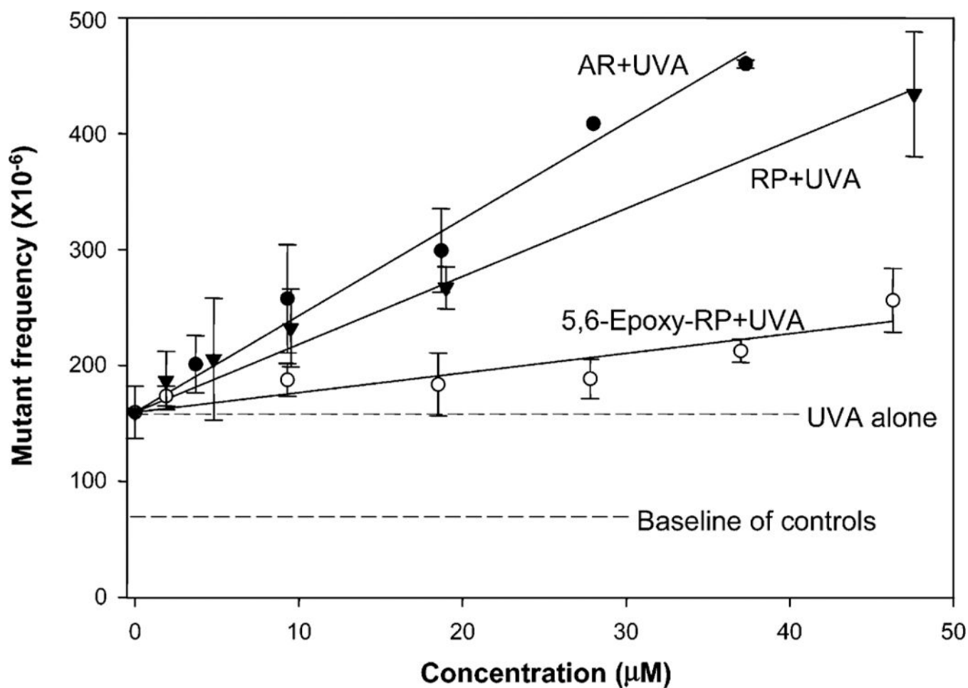
Figure 2. Comparison of photomutagenicity of RP (▼), AR (●), and 5,6-epoxy-RP (O) in mouse lymphoma cells. The cells were treated with different concentrations of compounds in conjunction with UVA irradiation of 2.48 J/cm 2 (1.38 mW/cm 2 for 30 min). The data points for AR + UVA and 5,6-epoxy-RP + UVA represent the mean of two independent experiments from Table 1. The RP + UVA data were from our previous results (19). UVA alone was the mean of mutant frequencies generated from all experiments with UVA treatment alone. The data for RP, AR, and 5,6-epoxy-RP were adjusted according to the mean of UVA alone as the origin of regression lines.
