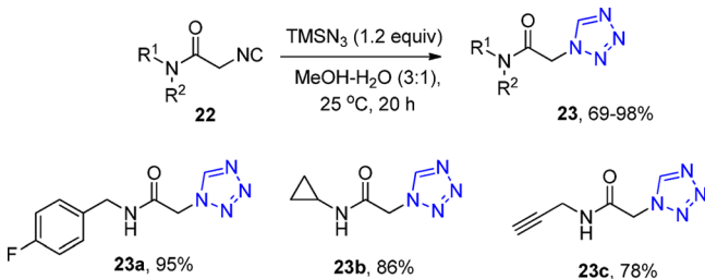
Scheme 6. Synthesis of 1-Substituted 1H-Tetrazoles 23 via N-Substituted Cyanoacetamides
