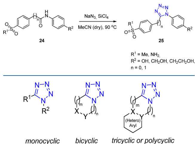
Figure 14. Classification of the MCR-based synthesis of tetrazole derivatives according to the number of cycles.
