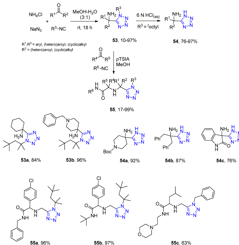
Scheme 16. A Synthetic Pathway to \alpha,\alpha -Disubstituted \alpha -Aminotetrazoles 53 and 54 Using an UT-4CR Employing Ammonium Chloride as an Ammonia Surrogate and the Post-Modification Towards Tetrazoles 55
