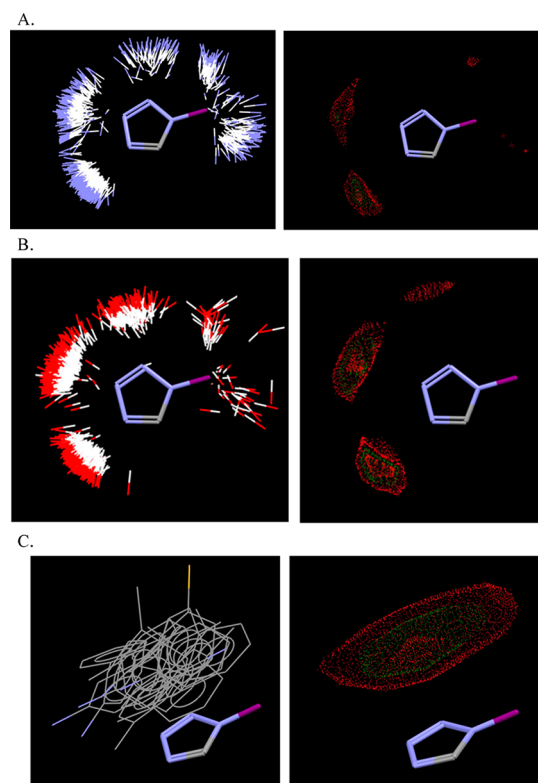
Figure 3. (A) The interactions of the 1,5-disubstituted 1H-tetrazoles with any N–H in CSD (2567 different plotted compounds, left). The majority of these interactions exists again around the two sp 2 3- and 4-nitrogens of the tetrazole ring as shown also by the contour surface (right). (B) The interactions of the 1,5-disubstituted 1H-tetrazoles with any O–H in CSD (2180 different plotted compounds, left). The majority of these interactions is distributed among the sp 2 nitrogens of the tetrazole ring and the N–H, respectively, as shown also by the contour surface (right). (C) π–π Interactions of the 1,5-disubstituted 1H-tetrazoles with phenyl rings, mostly in parallel-displaced stacking arrangement (left) as shown also by the contour surface (right) in CSD (946 different plotted compounds).
