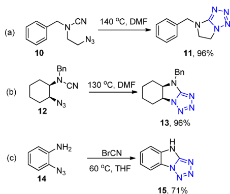
Scheme 4. Synthesis of 5-Substituted 1H-Tetrazoles 17 via N-Substituted Cyanoacetamides
