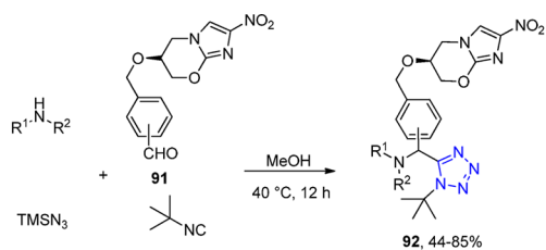
Scheme 34. Synthesis of New Nitroimidazole and Nitroimidazooxazine Derivatives 92
