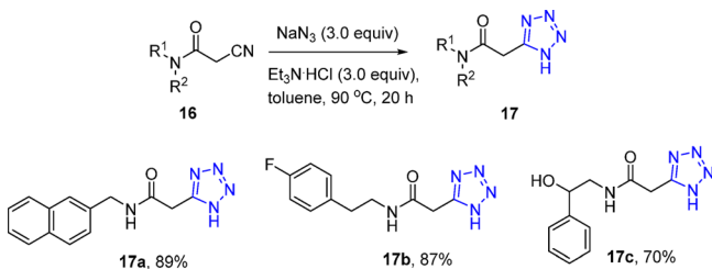
Scheme 4. Synthesis of 5-Substituted 1H-Tetrazoles 17 via N-Substituted Cyanoacetamides
