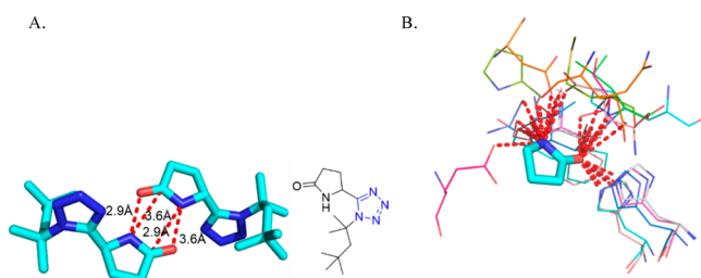
Figure 36. (A) Crystal structure of a tetrazolo fused \gamma -lactam 173a (CCDC 961190). It is worth mentioning that there is a pair wise hydrogen bonding with a neighbor lactam in short contacts (2.9 Å) between N6, O1 and N6', O1'. (B) Alignment of several PDB structures (3D23, 3EWJ, 3QZR, 3RHK, 3TNT, 3UR9, 3DPM, 1H0V, 3JUC, and 3Q3Y) showing the polar interactions for 10 \gamma -lactam containing ligands.
