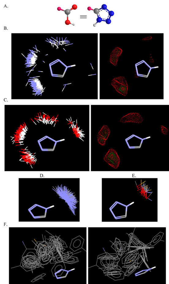
Figure 2. (A) Tetrazolic acids (5-substituted 1H-tetrazole or 2H-tetrazole) are bioisosteres of carboxylic acids. (B) The interactions of the 5-substituted 1H-tetrazoles with any N–H in CSD (655 different plotted compounds, left). The majority of these interactions exist around the two sp 2 3- and 4-nitrogens of the tetrazole ring as shown also by the contour surface (right). (C) The interactions of the 5-substituted 1H-tetrazoles with any O–H in CSD (696 different plotted compounds, left). The majority of these interactions is distributed among the sp 2 nitrogens of the tetrazole ring and the N–H, respectively, as shown also by the contour surface (right). (D) The interactions of the 5-substituted 1H-tetrazoles with aromatic or sp 2 N in CSD (1315 different plotted compounds), which demonstrate the acidic character of the N–H of the tetrazole. (E) Likewise, the interactions of the 5-substituted 1H-tetrazoles with terminal oxygen (carbonyl, amides, esters, acids, etc.) in CSD (159 different plotted compounds) depict the hydrogen bond formation of N–H⋯O=C. (F) π–π Interactions of the 5-substituted 1H-tetrazoles with phenyl rings (different poses in left and right picture) in T-shaped edge-to-face and parallel-displaced stacking arrangement in CSD (50 different plotted compounds).
