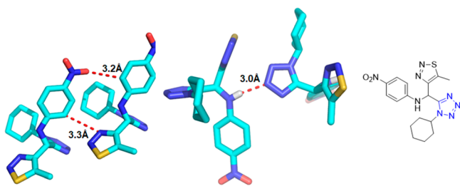
Figure 23. Crystal structure of N-((1\text{-cyclohexyl-1H-tetrazol-5-yl})(5\text{-methyl-1H-1,2,3-triazol-4-yl})\text{methyl})\text{-4-nitroaniline} (90d). It shows that the dihedral angles formed between the thiadiazole and tetrazole rings, the benzene and tetrazole rings, and the thiadiazole and benzene rings are 62.59^\circ , 86.73^\circ , and 70.07^\circ , respectively. Three intermolecular hydrogen bonds N(1)-H(2)\cdots N(6) , C(4)-H(4B)\cdots O(2) , and C(17)-H(17)\cdots N(3) are identified (CCDC 859295).
