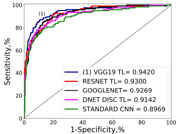
Fig. 4. Global performance comparison ROC curves and AUC values of the comparison of the networks of the study using the test set described in Table 5. The first option in terms of AUC is labeled as (1).
