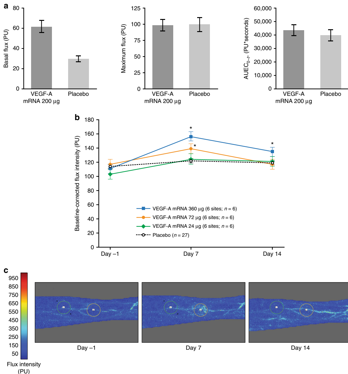
Fig. 4 Local skin blood flow outcomes. a Laser Doppler fluximetry 4 h after administration at VEGF-A mRNA injection sites and placebo sites (study part B, n = 15 ). Basal flux was measured before acetylcholine iontophoresis, and maximum flux and AUEC_{0-t} were measured after acetylcholine iontophoresis. b Laser Doppler imaging 7 and 14 days after administration (study part A, n = 27 ). Blue squares, VEGF-A mRNA 360 µg (6 sites; n = 6 ); orange circles, VEGF-A mRNA 72 µg (6 sites; n = 6 ); green diamonds, VEGF-A mRNA 24 µg (6 sites; n = 6 ); black circles, placebo (36 sites; n = 27 ). c Representative laser Doppler images showing the two injection sites at each time-point (study part A). Data are means with error bars showing SEM; * p < 0.05 , change from baseline (day -1) versus placebo (ad hoc mixed-effects repeated measurements model; nominal p values). AUEC_{0-t} , area under the effect curve from start to end of acetylcholine iontophoresis; PU, perfusion units; SEM, standard error of the mean; VEGF-A mRNA, vascular endothelial growth factor A modified messenger RNA
