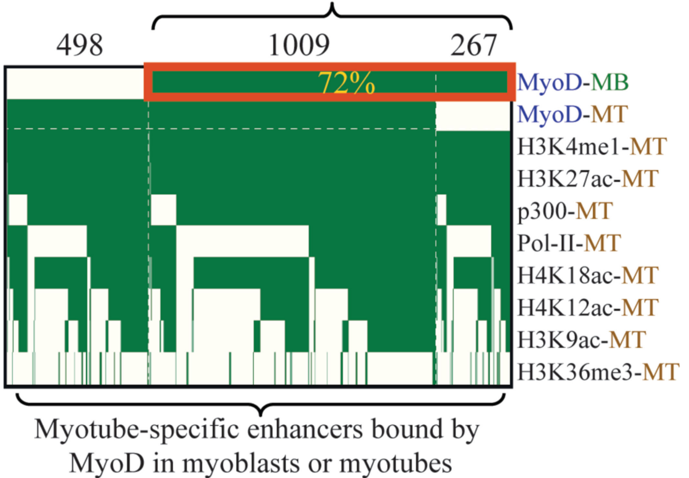
Figure 1: A large fraction of myotube-specific enhancer that is bound by MyoD, becomes bound by MyoD already in the proliferative stage.
