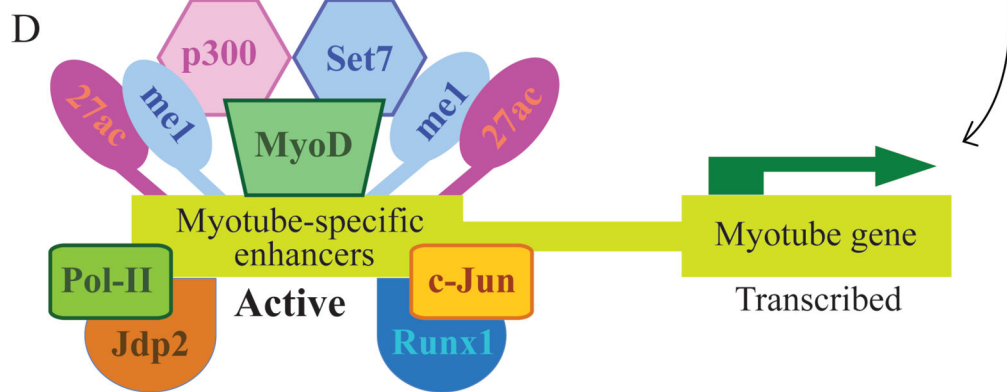
Figure 2: A hypothetical model for the involvement of placeholder in regulation of myotube-specific enhancer assembly and activation.
