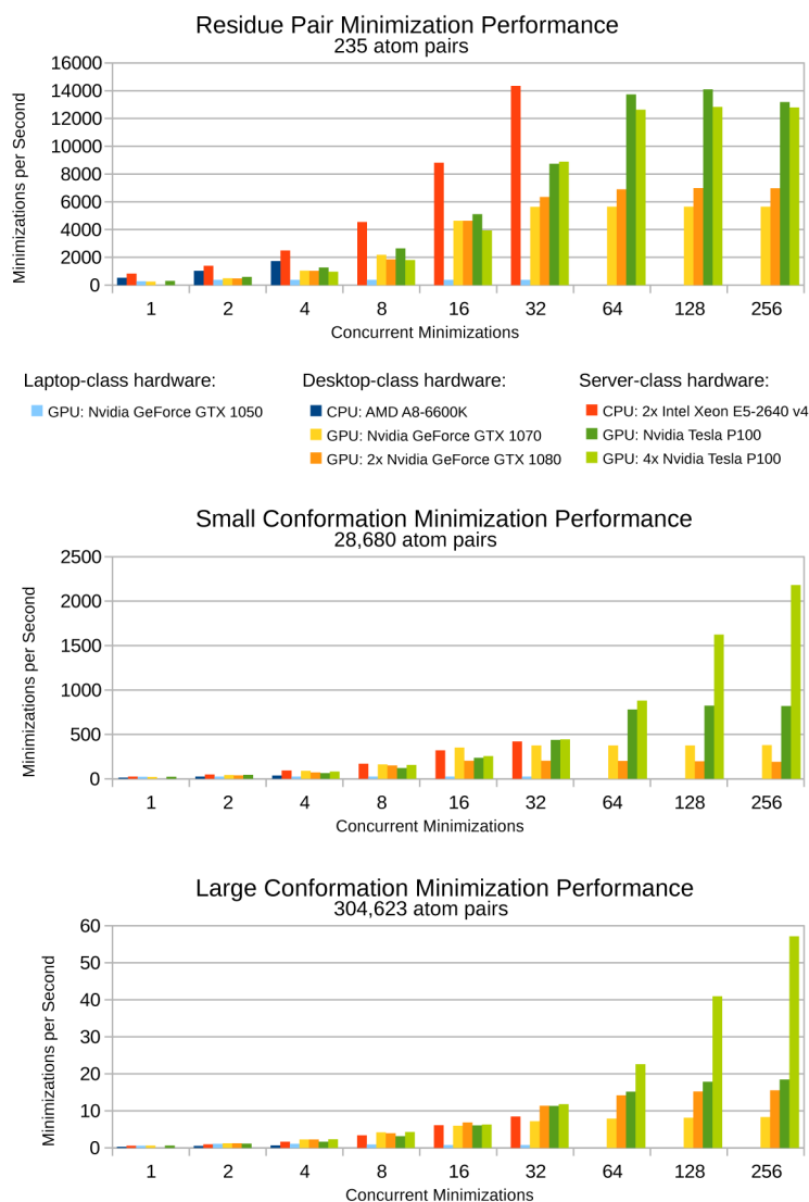
Figure 3: Benchmarks for protein conformation minimization in OSPREY 3.0 for various hardware platforms and for conformations of varying size.
