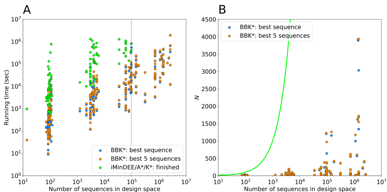
Figure 8: Measuring the contributions of the BBK^* 36 algorithmic improvements to the empirically observed running times of OSPREY.
