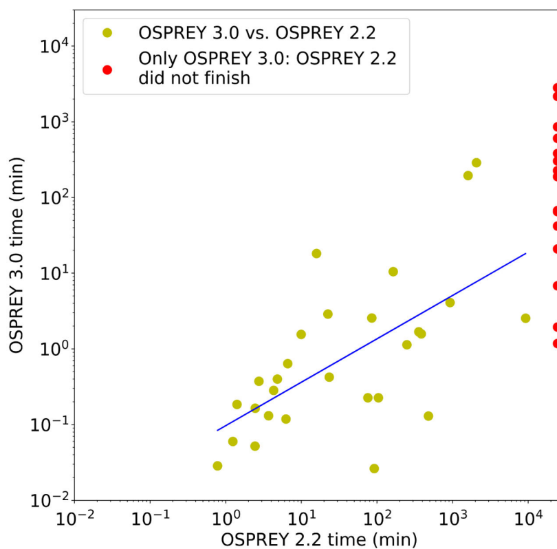
Figure 2: Runtimes of OSPREY 2.2 vs. OSPREY 3.0 for 45 protein design test cases (details shown in Table 1), shown on a log scale.
