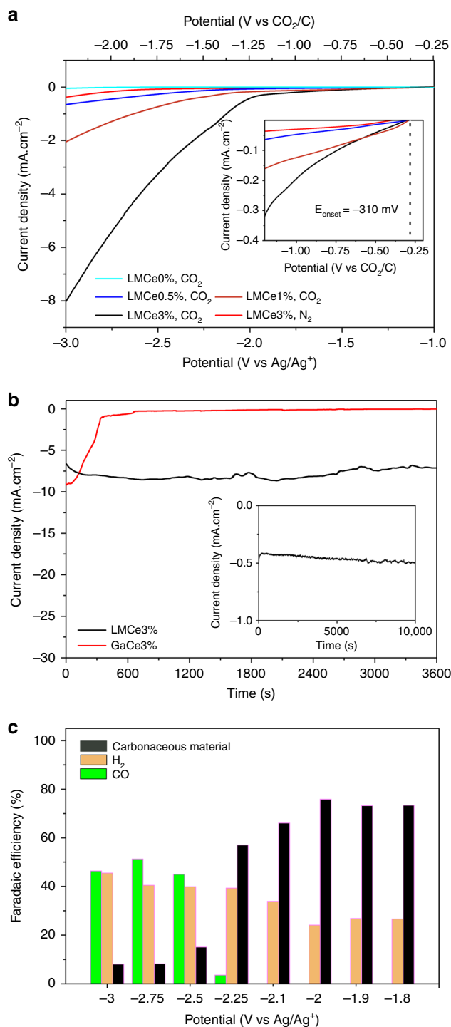
Fig. 1 Characteristics of CO_2 reduction by the LM Ce electrocatalyst. a linear sweep voltammogram (LSV) of galinstan with different concentrations of Ce measured in 0.1 M tetrabutylammonium hexafluorophosphate (TBAPF 6 ) and 2 M H_2O in dimethylformamide (DMF) in N_2 and CO_2 saturated electrolyte. Inset shows a magnified view. b Chrono-amperometry results of liquid galinstan and solid gallium containing 3% Ce measured at -3 V vs. Ag/Ag^+ in CO_2 saturated electrolyte. Inset shows chrono-amperometry result of a liquid galinstan alloy containing 3 wt% Ce (LMCe3%) at -2 V vs. Ag/Ag^+ in CO_2 saturated electrolyte. Please note the Faradaic efficiency for the various products at -2 and -3 V vs. Ag/Ag^+ which is shown in c . c Faradaic efficiencies of LMCe3% for the production of CO , H_2 , and solid carbonaceous material at corresponding potentials measured in CO_2 saturated electrolytes. The Faradaic efficiency for the carbonaceous material was determined via a deduction process. Please refer to the Methods section for further details
