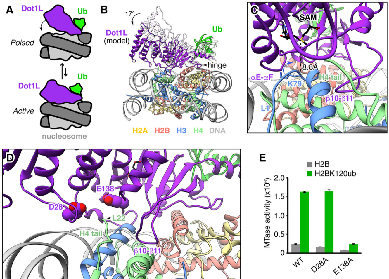
Figure 4. Model of Active Conformation of Dot1L on the Nucleosome
