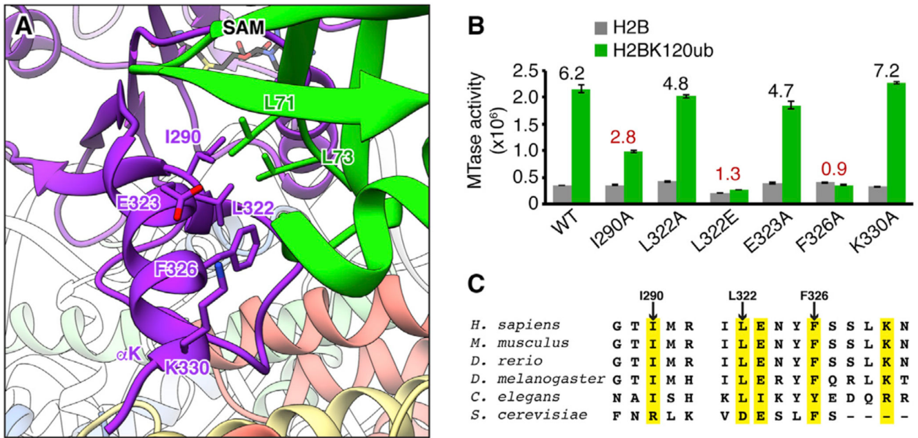
Figure 3. Ubiquitin Interacts with Dot1L to Enhance H3K79 Methylation
