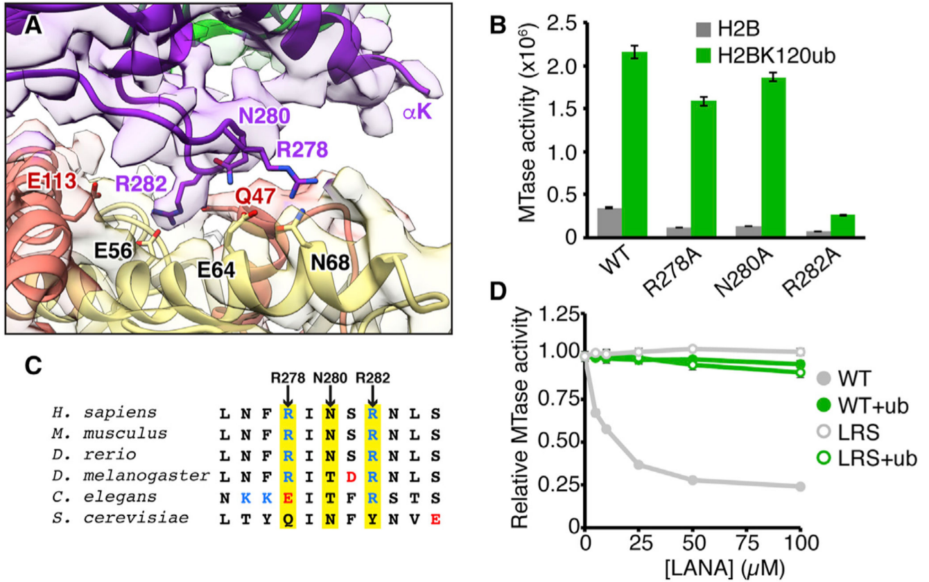
Figure 2. Dot1L Interacts with the Nucleosome Acidic Patch
