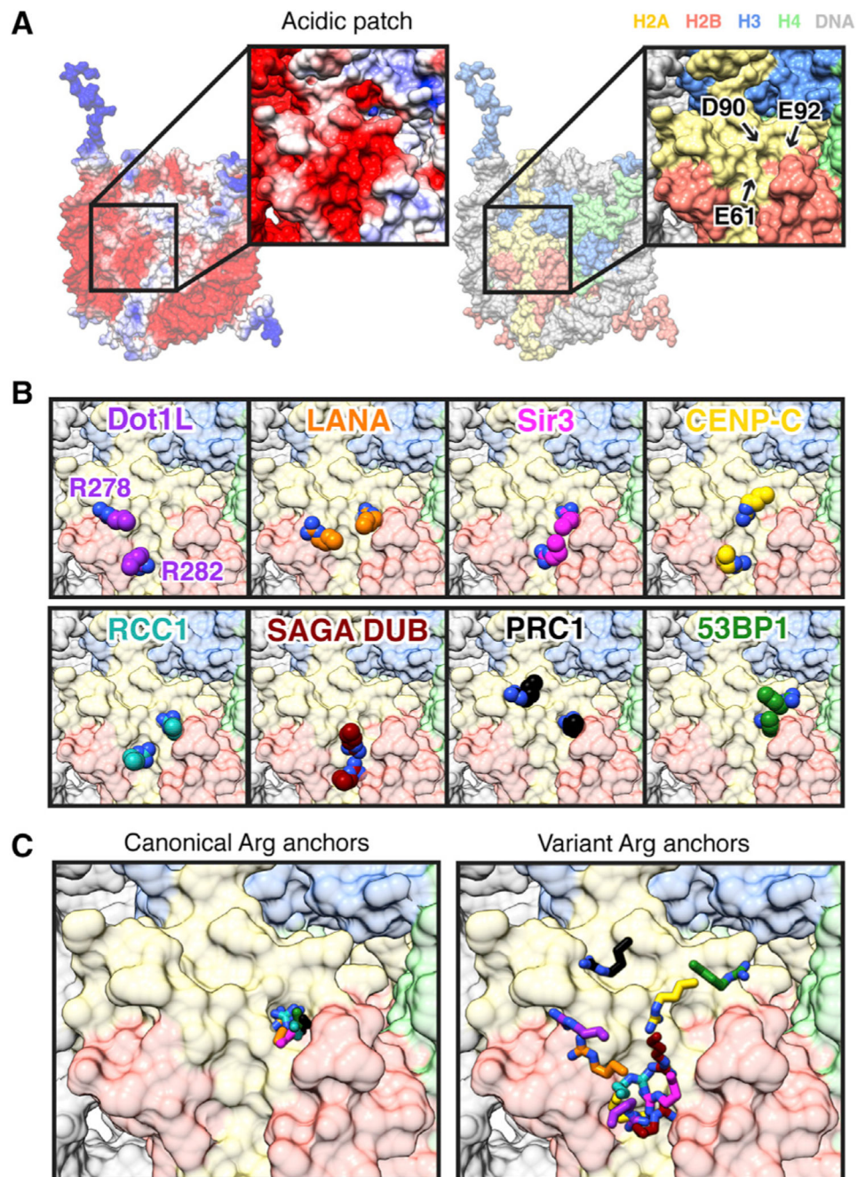
Figure 5. Canonical and Variant Arginine Anchors Bind the Nucleosome Acidic Patch (A) Electrostatic (generated with Adaptive Poisson-Boltzmann Solver [APBS] using AMBER) and histone-colored surfaces of nucleosome. (B) Zoomed views of arginine anchors of Dot1L, LANA (PDB: 1ZLA), Sir3 (PDB: 3TU4), CENP-C (PDB: 4X23), RCC1 (PDB: 3MVD), SAGA DUB module (PDB: 4ZUX), PRC1/RING1B (PDB: 4RP8), and 53BP1 (PDB: 5KGF). (C) Overlay of all canonical (left) and variant (right) arginine anchors.
