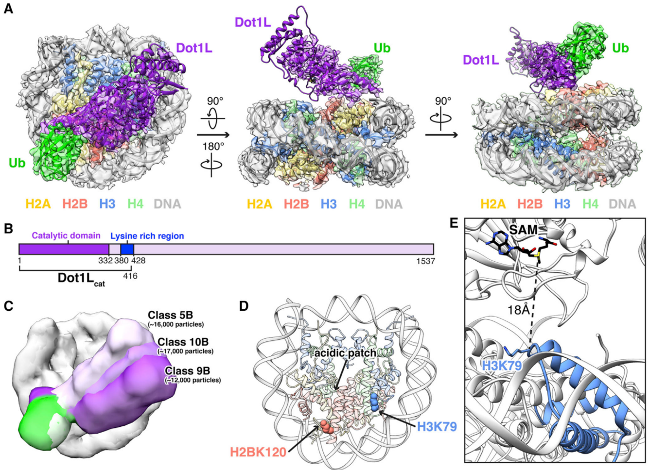
Figure 1. Cryo-EM Structure of Dot1L-H2BK120ub Nucleosome Complex
