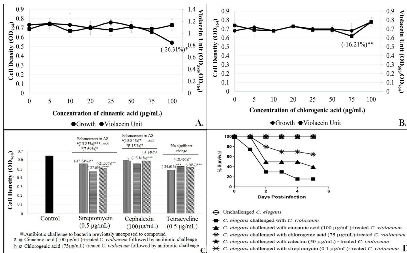
Figure 5. Effect of cinnamic acid and chlorogenic acid on C. violaceum . 'Control' in this figure is the vehicle control (0.5%v/v DMSO), which did not exert any effect on growth and violacein production of C. violaceum . (A) Effect of cinnamic acid on growth and violacein production in C. violaceum . Bacterial growth was measured as OD 764 ; OD of violacein was measured at 585 nm, and Violacein Unit was calculated as the ratio OD 585 /OD 764 (an indication of violacein production per unit of growth). (B) Effect of chlorogenic acid on growth and violacein production in C. violaceum . Bacterial growth was measured as OD 764 ; OD of violacein was measured at 585 nm, and violacein unit was calculated as the ratio OD 585 /OD 764 (an indication of violacein production per unit of growth). (C) Pre-treatment of C. violaceum with chlorogenic acid and cinnamic acid enhances its susceptibility to streptomycin and cephalixin. (D) Cinnamic acid, chlorogenic acid, and catechin reduced virulence of C. violaceum towards C. elegans . Catechin (50 µg/ml) and ampicillin (500 µg/ml) employed as positive controls conferred 100% protection on worm population. DMSO present in the 'vehicle control' at 0.5%v/v did not affect virulence of the bacterium towards C. elegans ; DMSO (0.5%v/v) and compounds at tested concentrations showed no toxicity towards the worm. * p <0.05, ** p <0.01, *** p <0.001. AS, antibiotic susceptibility; QS, quorum sensing.
