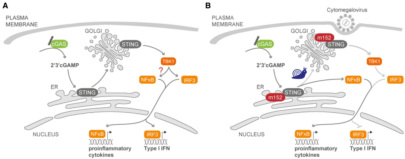
Figure 9. The multifaceted m152 protein selectively modulates STING-dependent type I IFN, but not NF-κB, signaling.
