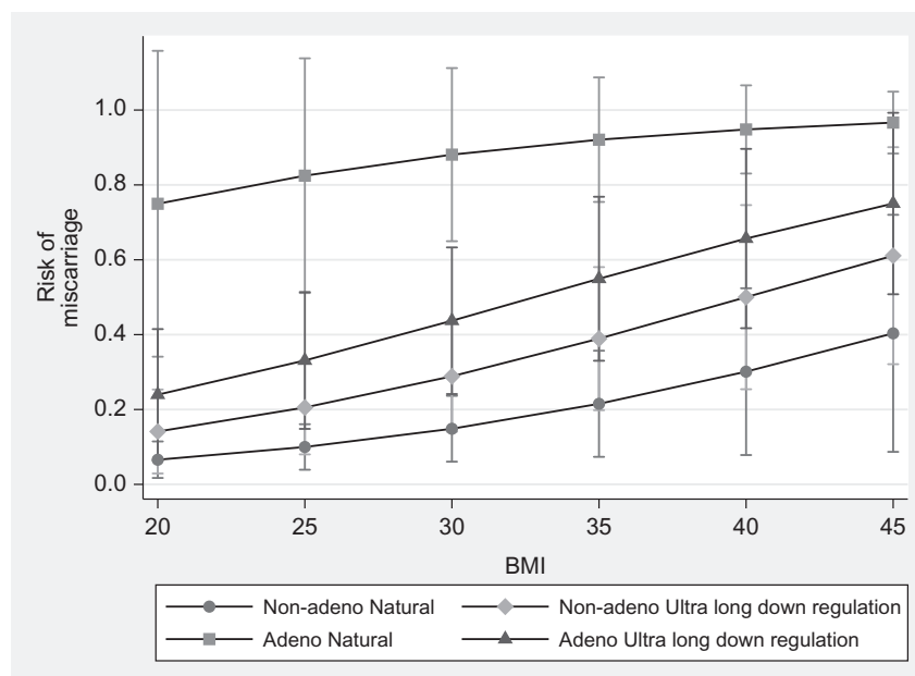
Figure 2 Predicted risk of miscarriage as a function of adenomyosis status The (marginal) predicted probabilities were obtained using binary logistic regression with age, BMI, log-transformed HCGUI, adenomyosis and an interaction term for adenomyosis × BMI.
