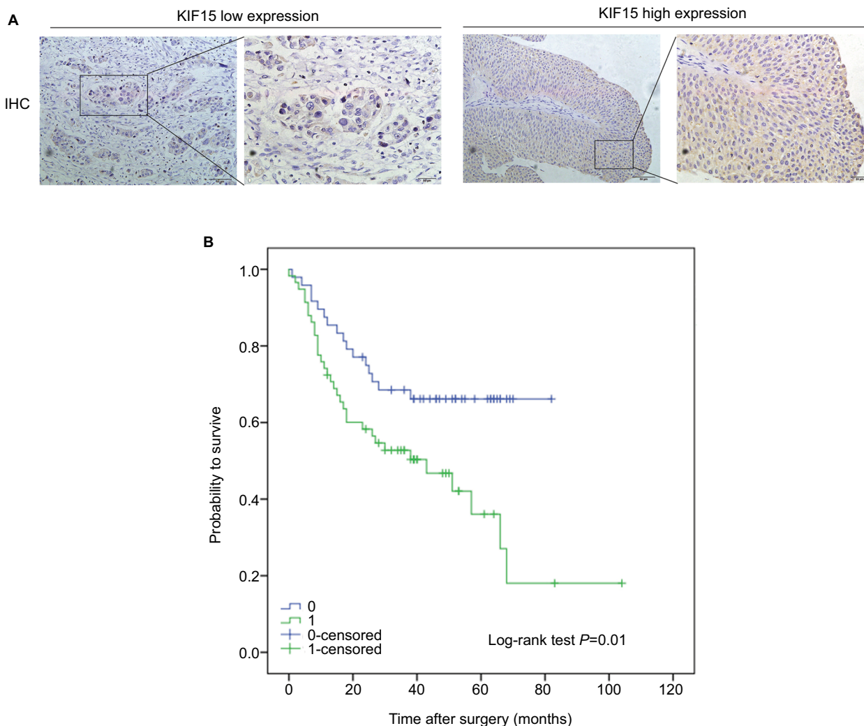
Figure 4 Correlation of KIF15 expression with clinicopathological characteristics and prognosis of bladder cancer patients.
