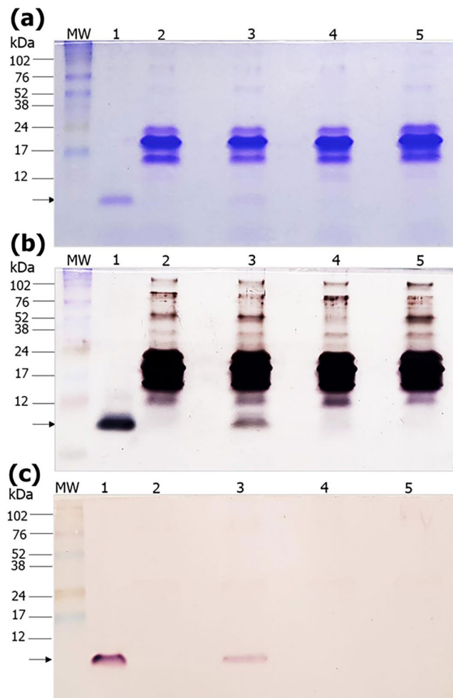
Figure 1. SDS-PAGE and Western blot analysis of mice urine samples. Urine of mice treated daily with vehicle saline or crotonamine, by intraperitoneal ( ip ) route 1.5 h before urine collection, were applied to a 15% SDS-PAGE before the (a) staining with Coomassie blue, (b) silver staining, or (c) Western blot analysis with anti-crotonamine antibody followed by development with alkaline phosphatase substrates NBT/BCIP. The presence of a protein band of about 5 kDa, corresponding to the full-length crotonamine, is indicated by the arrows. MW: molecular weight markers (kDa), lane 1: native crotonamine (100 ng), lane 2: urine of drug-naïve mouse receiving a single injection of vehicle saline (100 µL/animal), lane 3: urine of drug-naïve mouse receiving a single injection of native crotonamine (30 µg/100 µL/animal), lane 4: urine of negative control mice treated daily with vehicle (100 µL/animal) for 21 days, and lane 5: urine of mice treated daily with crotonamine (1 µg/100 µL/animal) for 21 days. In each lane, 5 µL of urine sample were loaded. The gels (a and b) and blot (c) are cropped along the edges. Complete uncropped blots/gels are presented in Supplementary Figure 3.
