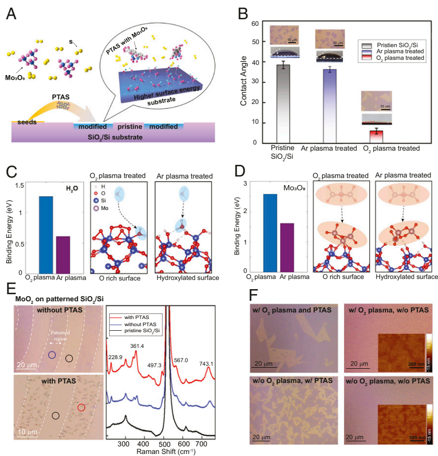
Fig. 2. Mechanism study for the patterned growth of monolayer \text{MoS}_2 nanostructures. (A) Schematic illustration of the growth mechanism of the patterned growth of \text{MoS}_2 . (B) Comparison of contact angles for pristine, Ar plasma-treated, and \text{O}_2 plasma-treated \text{SiO}_2/\text{Si} substrates. (C) DFT calculation for the binding energies between \text{H}_2\text{O} and \text{SiO}_2/\text{Si} substrate treated by \text{O}_2 plasma and Ar plasma. (D) DFT calculation for the binding energies between \text{Mo}_3\text{O}_9 and \text{SiO}_2/\text{Si} substrate treated by \text{O}_2 plasma and Ar plasma. (E, Upper Left) OM image of \text{MoO}_2 particles preferentially deposited on patterned \text{SiO}_2/\text{Si} regions without PTAS. (E, Lower Left) OM image of \text{MoO}_2 particles preferentially deposited on patterned \text{SiO}_2/\text{Si} regions with the presence of PTAS. (E, Right) Raman spectra collected at the regions indicated by the red, blue, and black circles in the OM images in Left; several \text{MoO}_2 Raman peaks are labeled in the spectra. It is shown that \text{MoO}_2 particles exhibit a clear preference to deposit on the patterned region and that the Raman peaks of \text{MoO}_2 are stronger with the presence of PTAS. (F, Upper Left) OM image of monolayer \text{MoS}_2 flakes grown on \text{O}_2 plasma-treated \text{SiO}_2/\text{Si} substrate with the assistance of PTAS. The domain size of \text{MoS}_2 is around 20\ \mu\text{m} . (F, Upper Right) OM image of small \text{MoS}_2 flakes grown on \text{O}_2 plasma-treated \text{SiO}_2/\text{Si} substrate without PTAS. (Inset) AFM images of \text{MoS}_2 small flakes with domain size around 300\ \text{nm} . (F, Lower Left) OM image of monolayer \text{MoS}_2 flakes grown on pristine \text{SiO}_2/\text{Si} substrate with the assistance of PTAS. The domain size of \text{MoS}_2 is around 8\text{--}10\ \mu\text{m} . (F, Lower Right) OM image of small \text{MoS}_2 flakes grown on pristine \text{SiO}_2/\text{Si} substrate without PTAS seed. (Inset) AFM images of \text{MoS}_2 small flakes with domain size around 200\ \text{nm} , indicating the poor quality of \text{MoS}_2 growth.
