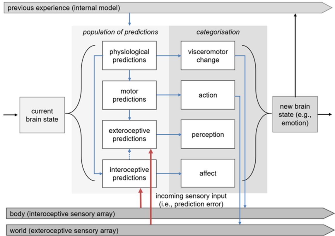
Figure 1. Schematic depiction of the dynamics of a mental event (e.g., an instance of emotional experience) from prediction to categorisation. Blue lines indicate top-down signal; red lines indicate bottom-up signal. Based on the current brain state, previous experience is used to generate a cascade of predictions focused on meeting the body’s expected needs for action (i.e., allostasis). As depicted, changes in sensory input (i.e., prediction error) may result in further tuning of the predictions. When predictions are confirmed, the current sensory array has been categorised and a new brain state instantiated. In turn, visceromotor changes and actions impact sensory inputs from the body and world, respectively. Current experience also updates the internal model, becoming part of the previous experience that will be brought to bear in future predictions.
