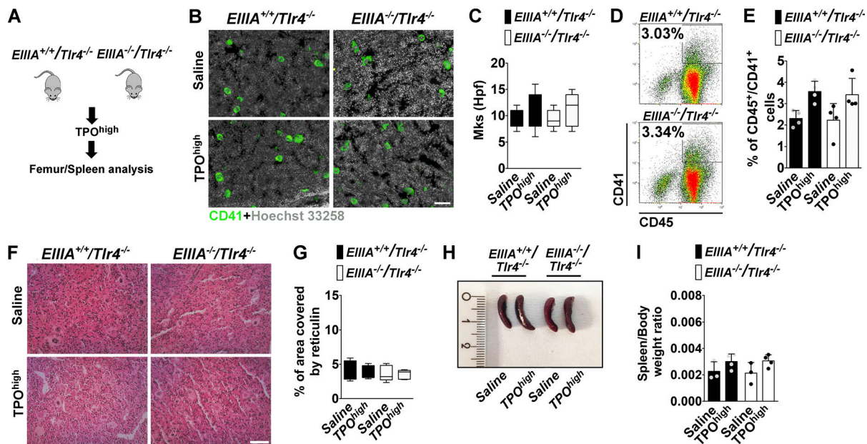
Figure 7. Response of EIIIA ^{+/+} /Tlr4 ^{-/-} and EIIIA ^{-/-} /Tlr4 ^{-/-} mice to TPO confirmed the critical role of EDA FN-TLR4 axis in BM fibrosis. (A) The TPO high model was established in EIIIA ^{+/+} /Tlr4 ^{-/-} and EIIIA ^{-/-} /Tlr4 ^{-/-} mice. (B and C) Representative immunofluorescence of BM CD41 ^+ Mk's (B) and quantification of Mk's per high power field (hpf); C) in EIIIA ^{+/+} /Tlr4 ^{-/-} and EIIIA ^{-/-} /Tlr4 ^{-/-} mice after treatment with TPO. Bar, 50 \mu m. Objective, 20 \times . (D and E) Representative flow cytometry dot plots (D) and relative quantification (E) of CD45/41 ^+ Mk's in BM cells of EIIIA ^{+/+} /Tlr4 ^{-/-} and EIIIA ^{-/-} /Tlr4 ^{-/-} mice after treatment with TPO. n = 4. (F and G) Gomori stain (F) and quantitative assessment of reticulin deposition (G) in treated mice. Bar, 50 \mu m. Objective, 20 \times . n = 3. (H) Representative spleens of saline- and TPO-treated EIIIA ^{+/+} /Tlr4 ^{-/-} and EIIIA ^{-/-} /Tlr4 ^{-/-} mice. (I) Quantification of spleen/body weight ratios in EIIIA ^{+/+} /Tlr4 ^{-/-} and EIIIA ^{-/-} /Tlr4 ^{-/-} mice treated with saline or TPO. n = 3 and 4, respectively. *, P < 0.05; **, P < 0.01; ***, P < 0.001. Data are shown as mean \pm SD.
